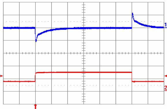
Fig. 1.2V.12: Output voltage response to load current step-change (3.75 A – 7.5 A – 3.75 A) at V_{in} = 24V . Top trace: output voltage (100 mV/div.). Bottom trace: load current (5 A/div.). Current slew rate: 5 A/ \mu s . C_o = 450 \mu F tantalum + 1 \mu F ceramic. Time scale: 0.2 ms/div.
