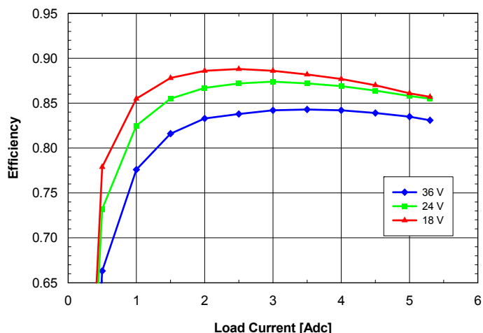
Fig. 8.0V.2: Efficiency vs. load current and input voltage for SQ24T/S05080 converter mounted vertically with air flowing from pin 3 to pin 1 at a rate of 300 LFM (1.5 m/s) and T_A = 25^\circ\text{C} .
