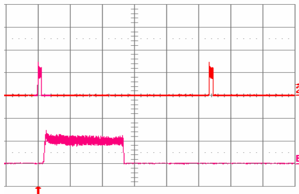
Fig. 12V.18: Load current (top trace, 5 A/div., 20 ms/div.) into a 10 mΩ short circuit during restart, at V_{in} = 24V . Bottom trace (5 A/div., 1 ms/div.) is an expansion of the on-time portion of the top trace.
