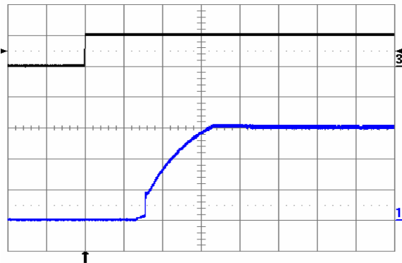
Fig. 1.5V.10: Turn-on transient at full rated load current (resistive) plus 10,000 \mu F at V_{in} = 24V , triggered via ON/OFF pin. Top trace: ON/OFF signal (5 V/div.). Bottom trace: output voltage (0.5 V/div.). Time scale: 1 ms/div.
