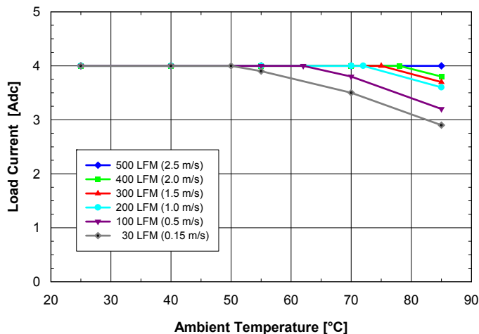
Fig. 12V.4: Available load current vs. ambient temperature and airflow rates for SQ24S04120 converter mounted horizontally with V_{in} = 24V , air flowing from pin 3 to pin 1 and maximum FET temperature \leq 120^{\circ}C .
