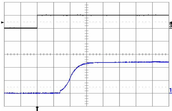
Fig. 12V.9: Turn-on transient at full rated load current (resistive) with no output capacitor at V_{in} = 24V , triggered via ON/OFF pin. Top trace: ON/OFF signal (5 V/div.). Bottom trace: output voltage (5 V/div.). Time scale: 1 ms/div.
