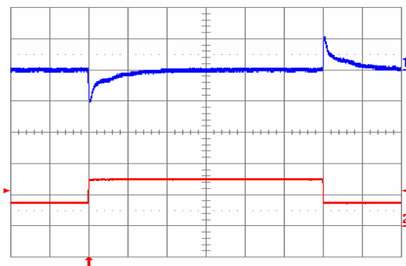
Fig. 3.3V.12: Output voltage response to load current step-change (3.75A – 7.5A – 3.75A) at V_{in} = 24V . Top trace: output voltage (100 mV/div.). Bottom trace: load current (5 A/div.). Current slew rate: 5 A/ \mu s . C_o = 450 \mu F tantalum + 1 \mu F ceramic. Time scale: 0.2 ms/div.
