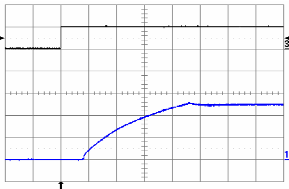
Fig. 5.0V.10: Turn-on transient at full rated load current (resistive) plus 10,000 \mu F at V_{in} = 24V , triggered via ON/OFF pin. Top trace: ON/OFF signal (5 V/div.). Bottom trace: output voltage (2 V/div.). Time scale: 2 ms/div.
