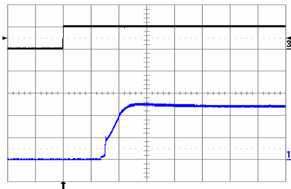
Fig. 1.2V.9: Turn-on transient at full rated load current (resistive) with no output capacitor at V_{in} = 24V , triggered via ON/OFF pin. Top trace: ON/OFF signal (5 V/div.). Bottom trace: output voltage (0.5 V/div.). Time scale: 1 ms/div.
