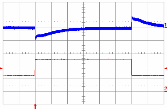
Fig. 5.0V.12: Output voltage response to load current step-change (2.5A – 5A – 2.5A) at V_{in} = 24V . Top trace: output voltage (100 mV/div.). Bottom trace: load current (2 A/div.). Current slew rate: 5 A/ \mu s . C_o = 450 \mu F tantalum + 1 \mu F ceramic. Time scale: 0.2 ms/div.
