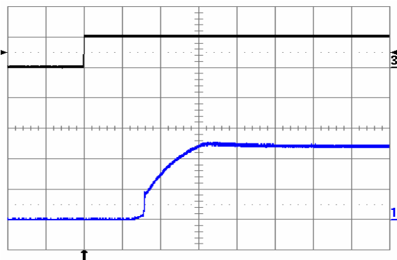
Fig. 1.2V.10: Turn-on transient at full rated load current (resistive) plus 10,000 \mu F at V_{in} = 24V , triggered via ON/OFF pin. Top trace: ON/OFF signal (5 V/div.). Bottom trace: output voltage (0.5 V/div.). Time scale: 1 ms/div.
