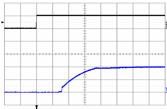
Fig. 2.0V.10: Turn-on transient at full rated load current (resistive) plus 10,000µF at V_{in} = 24V , triggered via ON/OFF pin. Top trace: ON/OFF signal (5 V/div.). Bottom trace: output voltage (1 V/div.). Time scale: 1 ms/div.
