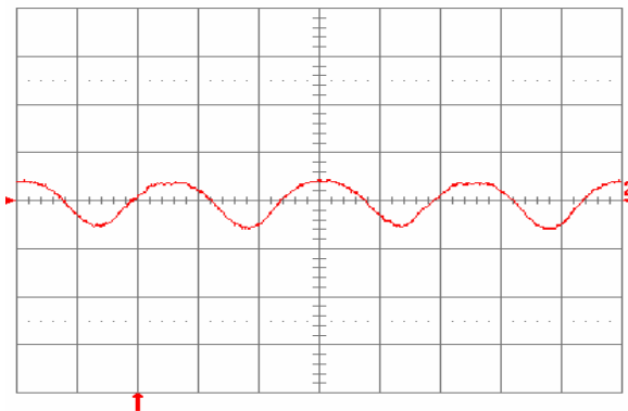
Fig. 1.5V.15: Input reflected ripple current, i_c (100 mA/div.), measured at input terminals at full rated load current and V_{in} = 24\text{V} . Refer to Fig. 1.5V.14 for test setup. Time scale: 1 \mu\text{s}/\text{div} .
