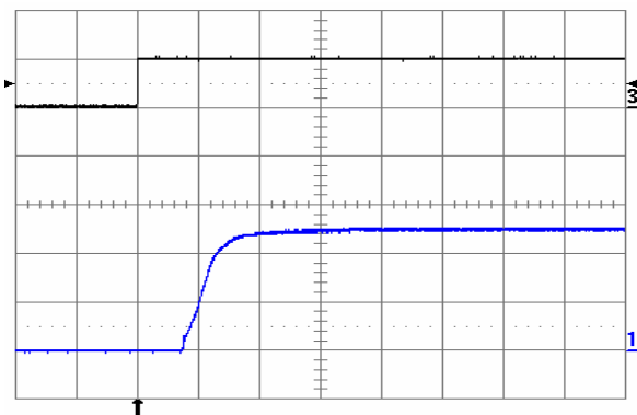
Fig. 5.0V.9: Turn-on transient at full rated load current (resistive) with no output capacitor at V_{in} = 24V , triggered via ON/OFF pin. Top trace: ON/OFF signal (5 V/div.). Bottom trace: output voltage (2 V/div.). Time scale: 2 ms/div.
