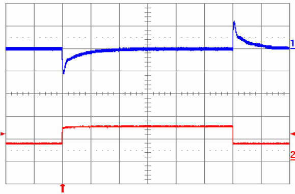
Fig. 1.5V.12: Output voltage response to load current step-change (3.75 A – 7.5 A – 3.75 A) at V_{in} = 24V . Top trace: output voltage (100 mV/div.). Bottom trace: load current (5 A/div.). Current slew rate: 5 A/ \mu s . C_o = 450 \mu F tantalum + 1 \mu F ceramic. Time scale: 0.2 ms/div.
