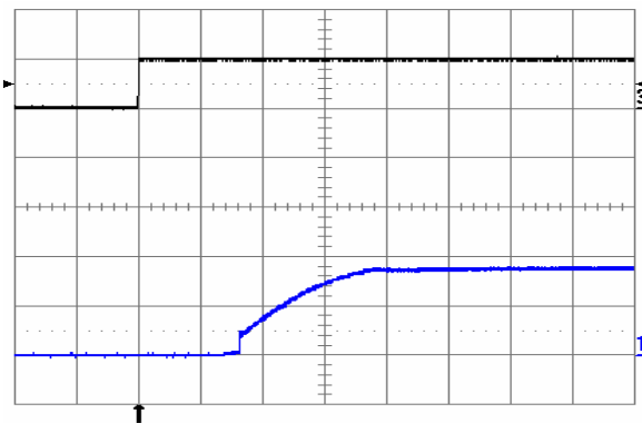
Fig. 1.8V.10: Turn-on transient at full rated load current (resistive) plus 10,000µF at V_{in} = 24V , triggered via ON/OFF pin. Top trace: ON/OFF signal (5 V/div.). Bottom trace: output voltage (1 V/div.). Time scale: 1 ms/div.
