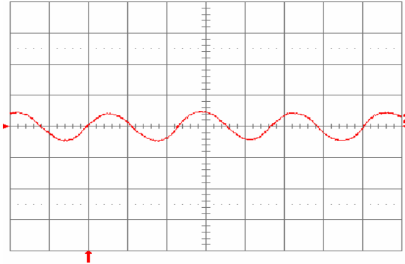
Fig. 2.5V.15: Input reflected ripple current, i_c (100 mA/div.), measured at input terminals at full rated load current and V_{in} = 24 \text{ V} . Refer to Fig. 2.5V.14 for test setup. Time scale: 1 \mu\text{s}/\text{div} .
