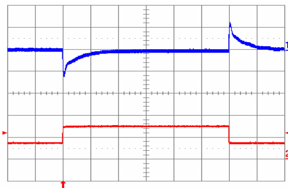
Fig. 2.0V.12: Output voltage response to load current step-change (3.75A – 7.5A – 3.75A) at V_{in} = 24V . Top trace: output voltage (100 mV/div.). Bottom trace: load current (5 A/div.). Current slew rate: 5 A/µs. C_o = 450 \mu F tantalum + 1 µF ceramic. Time scale: 0.2 ms/div.
