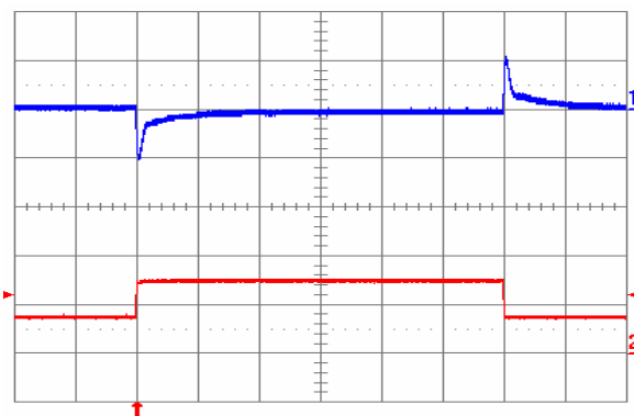
Fig. 1.8V.12: Output voltage response to load current step-change (3.75A – 7.5A – 3.75A) at V_{in} = 24V . Top trace: output voltage (100 mV/div.). Bottom trace: load current (5 A/div.). Current slew rate: 5 A/µs. C_o = 450 \mu F tantalum + 1 µF ceramic. Time scale: 0.2 ms/div.
