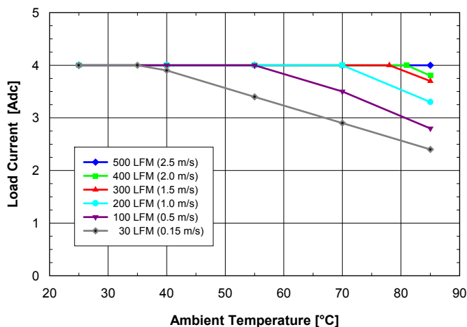
Fig. 12V.2: Available load current vs. ambient air temperature and airflow rates for SQ24T04120 converter with B height pins mounted horizontally with V_{in} = 24V , air flowing from pin 3 to pin 1 and maximum FET temperature \leq 120^{\circ}C .
