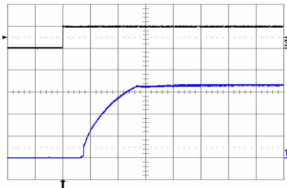
Fig. 3.3V.10: Turn-on transient at full rated load current (resistive) plus 10,000 \mu F at V_{in} = 24V , triggered via ON/OFF pin. Top trace: ON/OFF signal (5 V/div.). Bottom trace: output voltage (1 V/div.). Time scale: 2 ms/div.
