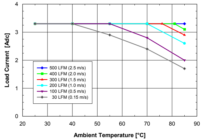
Fig. 2: Available load current vs. ambient air temperature and airflow rates for SQ24T03150 converter with B height pins mounted horizontally with V_{in} = 24 V, air flowing from pin 3 to pin 1 and maximum FET temperature \leq 120 °C.
