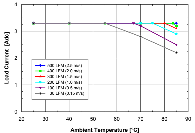
Fig. 4: Available load current vs. ambient temperature and airflow rates for SQ24S03150 converter mounted horizontally with V_{in} = 24 V, air flowing from pin 3 to pin 1 and maximum FET temperature \leq 120 °C.
