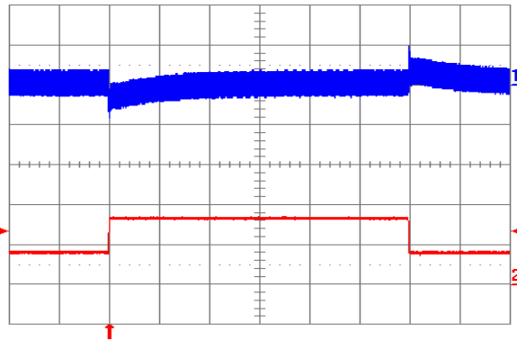
Fig. 11: Output voltage response to load current step-change (0.825 A – 1.65 A – 0.825 A) at V_{in} = 24 V. Top trace: output voltage (200 mV/div.). Bottom trace: load current (1 A/div.). Current slew rate: 0.1 A/ \mu s. C_o = 1 \mu F ceramic. Time scale: 0.5 ms/div.
