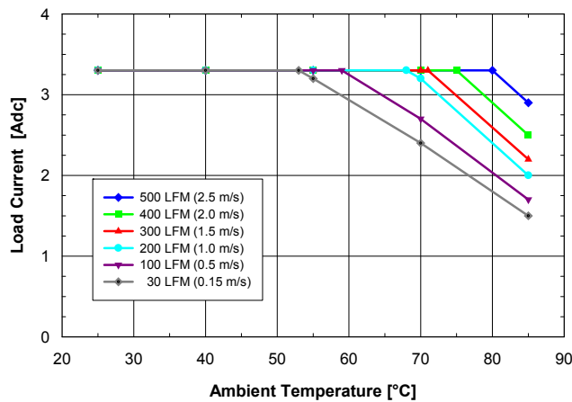
Fig. 1: Available load current vs. ambient air temperature and airflow rates for SQ24T03150 converter with B height pins mounted vertically with V_{in} = 24 V, air flowing from pin 3 to pin 1 and maximum FET temperature \leq 120 °C.
