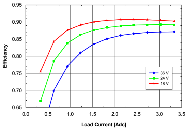
Fig. 5: Efficiency vs. load current and input voltage for SQ24T/S03150 converter mounted vertically with air flowing from pin 3 to pin 1 at a rate of 300 LFM (1.5 m/s) and T_a = 25\text{ }^{\circ}\text{C} .
