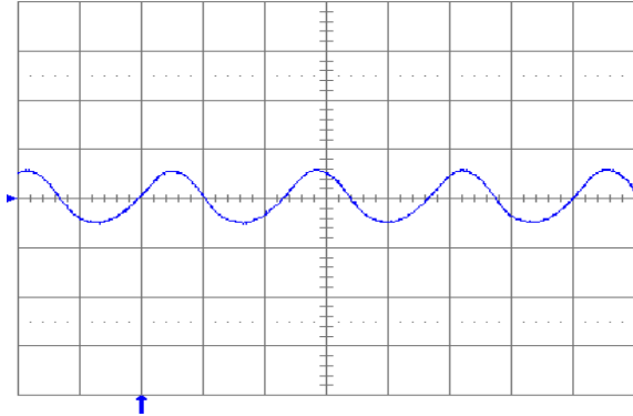
Fig. 13: Output voltage ripple (100 mV/div.) at full rated load current into a resistive load with C_o = 10 \mu\text{F} tantalum + 1uF ceramic and V_{in} = 24 \text{ V} . Time scale: 1 \mu\text{s}/\text{div} .
