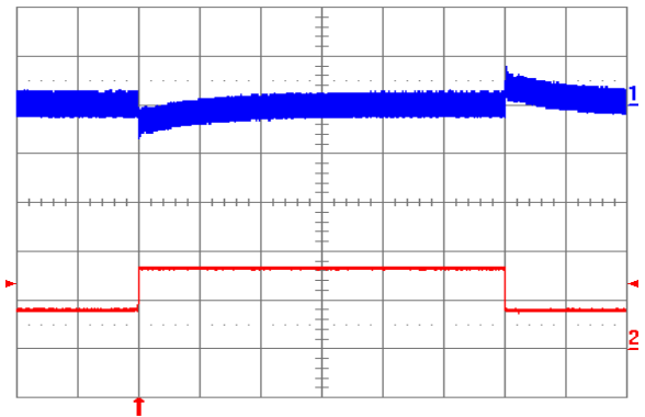
Fig. 12: Output voltage response to load current step-change (0.825 A – 1.65 A – 0.825 A) at V_{in} = 24 V. Top trace: output voltage (200 mV/div.). Bottom trace: load current (1 A/div.). Current slew rate: 5 A/ \mu s. C_o = 47 \mu F tantalum + 1 \mu F ceramic. Time scale: 0.5 ms/div.
