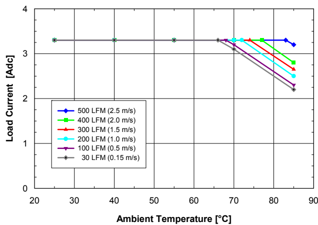
Fig. 3: Available load current vs. ambient temperature and airflow rates for SQ24S03150 converter mounted vertically with V_{in} = 24 V, air flowing from pin 3 to pin 1 and maximum FET temperature \leq 120 °C.
