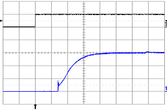
Fig. 9: Turn-on transient at full rated load current (resistive) with no output capacitor at V_{in} = 24 V, triggered via ON/OFF pin. Top trace: ON/OFF signal (5 V/div.). Bottom trace: output voltage (5 V/div.). Time scale: 1 ms/div.
