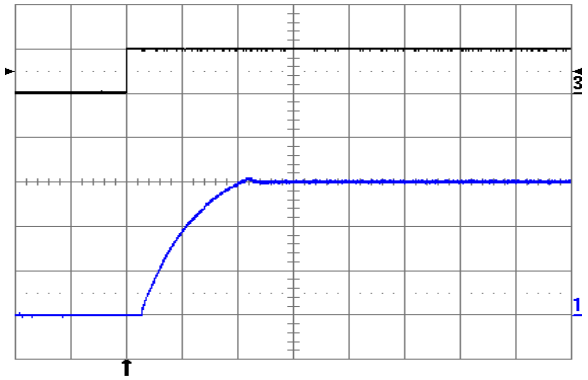
Fig. 10: Turn-on transient at full rated load current (resistive) plus 1,000 \mu F at V_{in} = 24 V, triggered via ON/OFF pin. Top trace: ON/OFF signal (5 V/div.). Bottom trace: output voltage (5 V/div.). Time scale: 5 ms/div.
