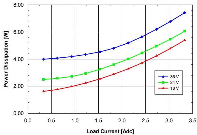
Fig. 7: Power dissipation vs. load current and input voltage for SQ24T/S03150 converter mounted vertically with air flowing from pin 3 to pin 1 at a rate of 300 LFM (1.5 m/s) and T_a = 25\text{ }^{\circ}\text{C} .
