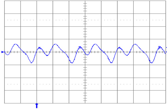
Fig. 1.2V.13: Output voltage ripple (20 mV/div.) at full rated load current into a resistive load with C_o = 10\ \mu\text{F} tantalum + 1\ \mu\text{F} ceramic and V_{in} = 24\ \text{V} . Time scale: 1\ \mu\text{s}/\text{div} .
