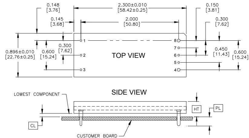
SQ24T Pinout (Through-hole)
