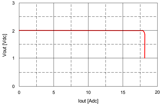
Fig. 2.0V.17: Output voltage vs. load current showing current limit point and converter shutdown point. Input voltage has almost no effect on current limit characteristic.
