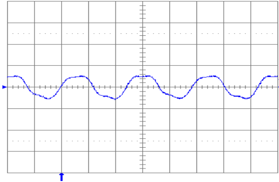
Fig. 6.0V.13: Output voltage ripple (50 mV/div.) at full rated load current into a resistive load with C_o = 10 \mu\text{F} tantalum + 1\mu\text{F} ceramic and V_{in} = 24 \text{ V} . Time scale: 1 \mu\text{s}/\text{div} .
