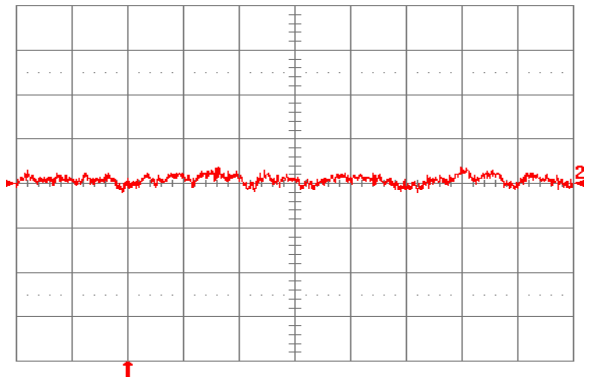
Fig. 1.0V.16: Input reflected ripple current, i_s (10 mA/div.), measured through 10 \mu\text{H} at the source at full rated load current and V_{in} = 24\text{V} . Refer to Fig. 1.0V.14 for test setup. Time scale: 1 \mu\text{s}/\text{div} .
