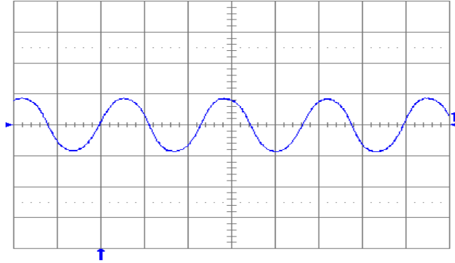
Fig. 12V.13: Output voltage ripple (50 mV/div.) at full rated load current into a resistive load with C_o = 10 \mu\text{F} tantalum + 1\mu\text{F} ceramic and V_{in} = 24 \text{ V} . Time scale: 1 \mu\text{s}/\text{div} .
