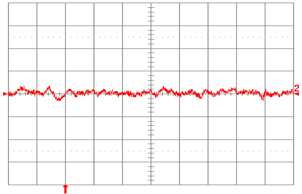
Fig. 2.5V.16: Input reflected ripple current, i_s (10 mA/div.), measured through 10 \mu\text{H} at the source at full rated load current and V_{in} = 24 \text{ V} . Refer to Fig. 2.5V.14 for test setup. Time scale: 1 \mu\text{s}/\text{div} .
