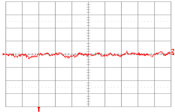
Fig. 3.3V.16: Input reflected ripple current, i_s (10 mA/div.), measured through 10 \mu\text{H} at the source at full rated load current and V_{in} = 24 \text{ V} . Refer to Fig. 3.3V.14 for test setup. Time scale: 1 \mu\text{s}/\text{div} .
