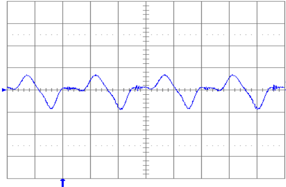
Fig. 1.5V.13: Output voltage ripple (20 mV/div.) at full rated load current into a resistive load with C_o = 10 \mu\text{F} tantalum + 1\mu\text{F} ceramic and V_{in} = 24 \text{ V} . Time scale: 1 \mu\text{s}/\text{div} .
