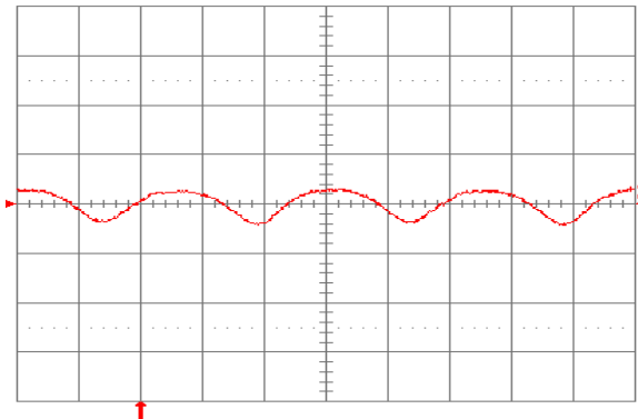
Fig. 1.0V.15: Input reflected ripple current, i_c (100 mA/div.), measured at input terminals at full rated load current and V_{in} = 24\text{V} . Refer to Fig. 1.0V.14 for test setup. Time scale: 1 \mu\text{s}/\text{div} .
