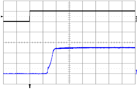
Fig. 2.5V.9: Turn-on transient at full rated load current (resistive) with no output capacitor at V_{in} = 24V , triggered via ON/OFF pin. Top trace: ON/OFF signal (5 V/div.). Bottom trace: output voltage (1 V/div.). Time scale: 1 ms/div.
