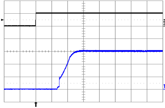
Fig. 1.5V.9: Turn-on transient at full rated load current (resistive) with no output capacitor at V_{in} = 24V , triggered via ON/OFF pin. Top trace: ON/OFF signal (5 V/div.). Bottom trace: output voltage (0.5 V/div.). Time scale: 1 ms/div.
