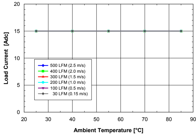
Fig. 1.0V.3: Available load current vs. ambient air temperature and airflow rates for SQ48S15010 converter mounted vertically with V_{in} = 48 V, air flowing from pin 3 to pin 1, and maximum FET temperature \leq 120 °C.
