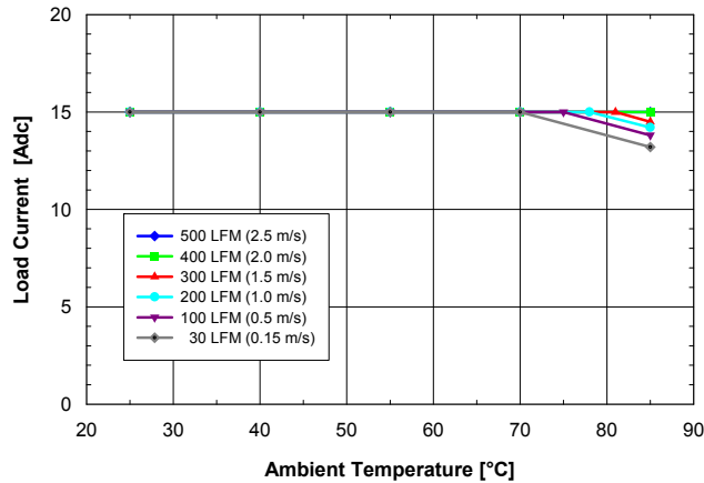
Fig. 1.8V.3: Available load current vs. ambient air temperature and airflow rates for SQ48S15018 converter mounted vertically with V_{in} = 48 V, air flowing from pin 3 to pin 1, and maximum FET temperature \leq 120 °C.
