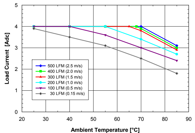
Fig. 12V.2: Available load current vs. ambient air temperature and airflow rates for SQ48T04120 converter with D height pins mounted horizontally with V_{in} = 48\text{ V} , air flowing from pin 3 to pin 1, and maximum FET temperature \leq 120^\circ\text{C} .
