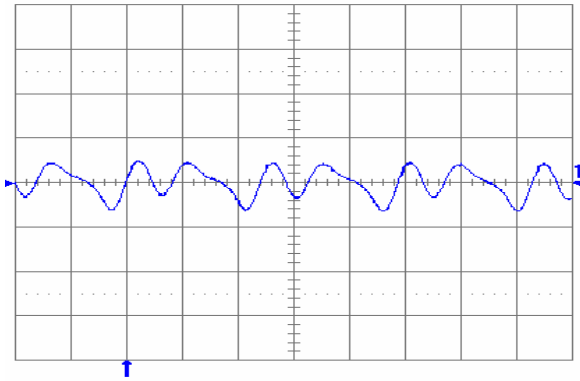
Fig. 1.0V.13: Output voltage ripple (20 mV/div.) at full rated load current into a resistive load with C_o = 10 μF tantalum + 1 μF ceramic and V_{in} = 48 V. Time scale: 1 μs/div.
