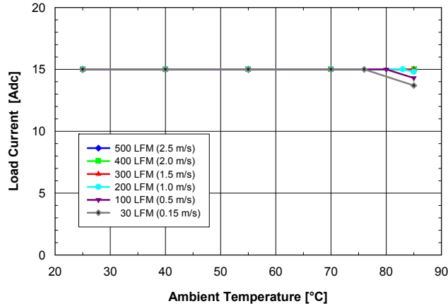
Fig. 1.5V.3: Available load current vs. ambient air temperature and airflow rates for SQ48S15015 converter mounted vertically with V_{in} = 48 V, air flowing from pin 3 to pin 1, and maximum FET temperature \leq 120 °C.
