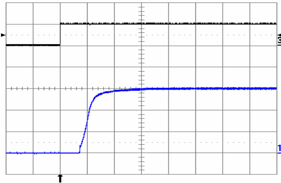
Fig. 6.0V.9: Turn-on transient at full rated load current (resistive) with no output capacitor at V_{in} = 48\text{ V} , triggered via ON/OFF pin. Top trace: ON/OFF signal (5 V/div.). Bottom trace: output voltage (2 V/div.). Time scale: 2 ms/div.
