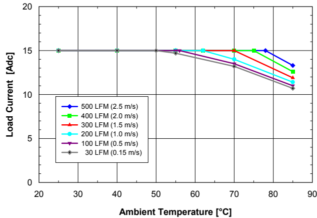
Fig. 2.5V.3: Available load current vs. ambient air temperature and airflow rates for SQ48S15025 converter mounted vertically with V_{in} = 48 V, air flowing from pin 3 to pin 1, and maximum FET temperature \leq 120 °C.
