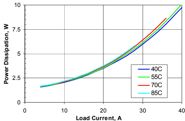
Figure 5. Power dissipation vs. load current and ambient temperature for SQE48T40015 converter mounted vertically with V_{in} = 48\text{ V} and air flowing from pin 3 to pin 1 at a rate of 200 LFM (1.0 m/s).
