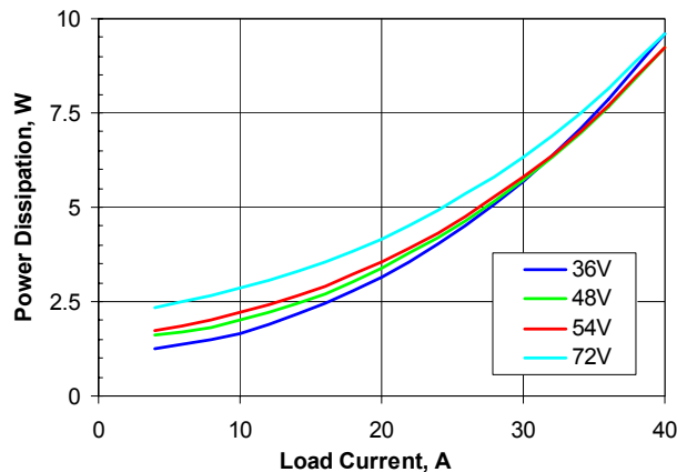
Figure 4. Power dissipation vs. load current and input voltage for SQE48T40015 converter mounted vertically with air flowing from pin 3 to pin 1 at a rate of 300 LFM (1.5 m/s) and T_a = 25^\circ\text{C} .
