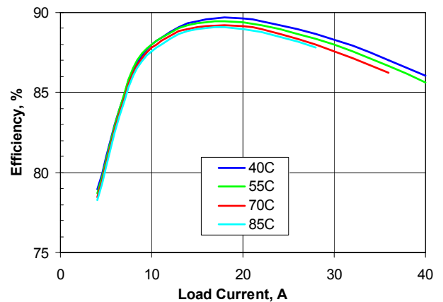
Figure 3. Efficiency vs. load current and ambient temperature for SQE48T40015 converter mounted vertically with V_{in}=48\text{ V} and air flowing from pin 3 to pin 1 at 200LFM (1.0m/s).
