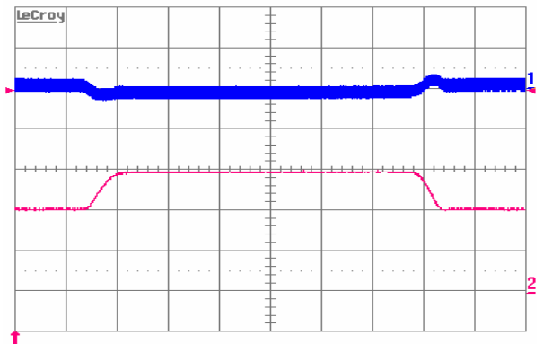
Figure 8. Output voltage response to load current step-change (20 A – 30 A – 20 A) at V_{in} = 48\text{ V} . Top trace: output voltage (100 mV/div.). Bottom trace: load current (10 A/div.). Current slew rate: 0.1 A/ \mu\text{s} . C_o = 1\text{ }\mu\text{F} ceramic. Time scale: 0.2ms/div.
