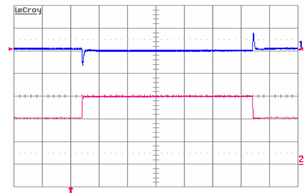
Figure 9. Output voltage response to load current step-change (20 A – 30 A – 20A) at V_{in} = 48\text{ V} . Top trace: output voltage (200 mV/div.). Bottom trace: load current (10 A/div.). Current slew rate: 2.5 A/ \mu\text{s} . C_o = 470\text{ }\mu\text{F POS} + 1\text{ }\mu\text{F} ceramic. Time scale: 0.2 ms/div.
