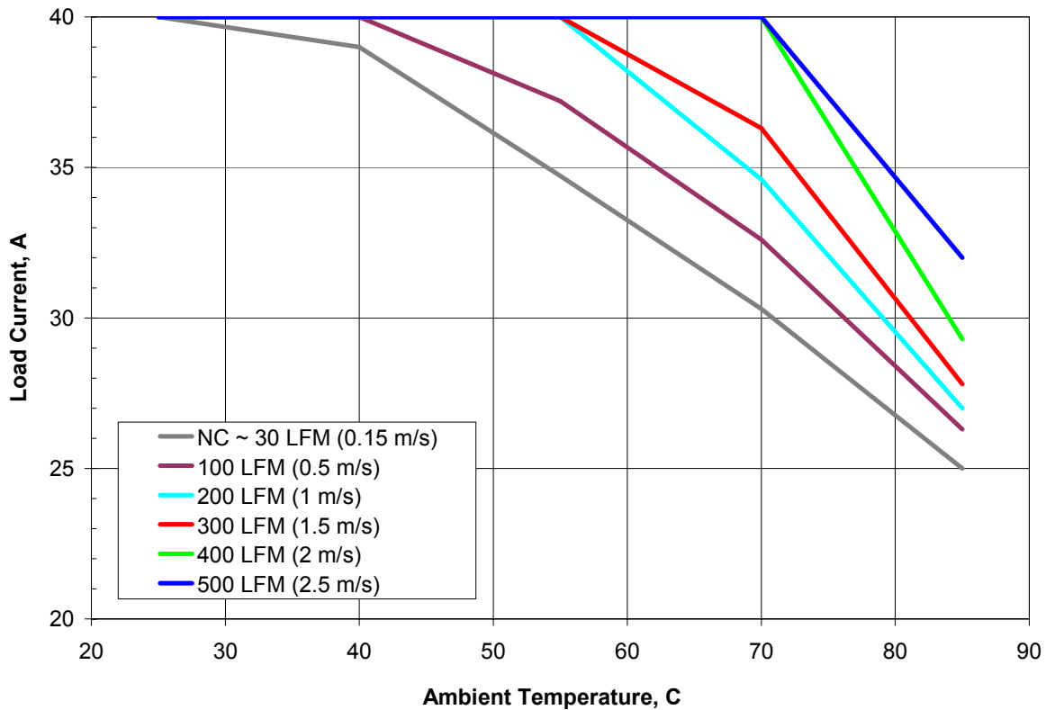
Figure 1. Available load current vs. ambient air temperature and airflow rates for SQE48T40015 converter mounted vertically with air flowing from pin 3 to pin 1, MOSFET temperature \leq 120\text{ }^{\circ}\text{C} , V_{in} = 48\text{ V} . Note: NC – Natural convection
