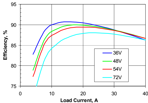
Figure 2. Efficiency vs. load current and input voltage for SQE48T40015 converter mounted vertically with air flowing from pin 3 to pin 1 at 300 LFM (1.5 m/s) and T_a=25^{\circ}\text{C} .
