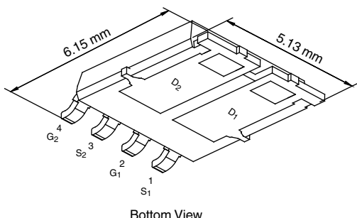
PowerPAK® SO-8L Dual
