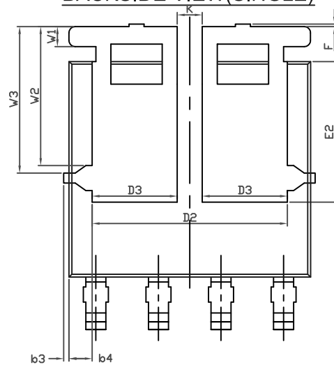
BACKSIDE VIEW(DUAL)
