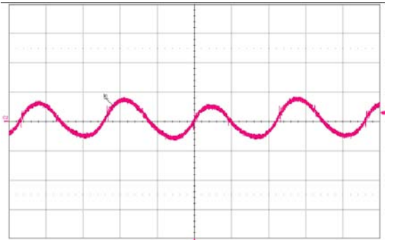
Figure 15. Input reflected ripple-current, i_c (100 mA/div.), measured at input terminals at full rated load current and V_{in} = 48 V. Refer to Fig. J for test setup. Time scale: 1 \mu s/div.
