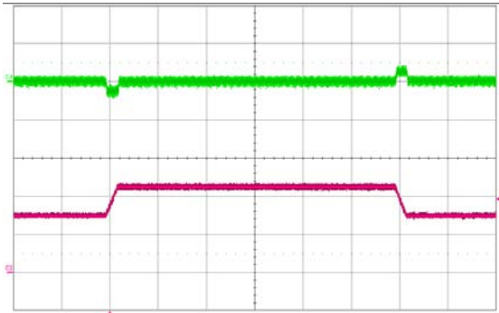
Figure 11. Output voltage response to load current step change (7.5A – 11.25A – 7.5A) at V_{in} = 48 V. Top trace: output voltage (50mV/div.) Bottom: load current (5 A/div.). Current slew rate: 0.1 A/ \mu s. Time scale: 200 \mu s /div. C_o = 10\mu F tantalum + 1 \mu F ceramic
