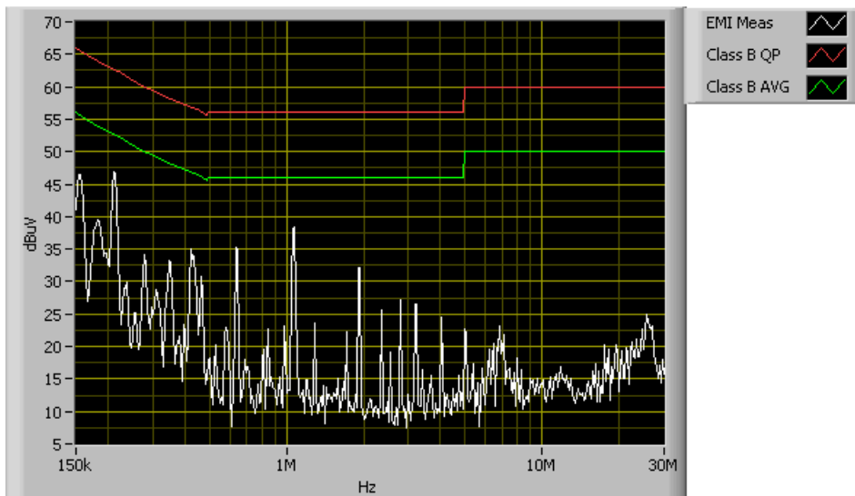
EMI Measurement
