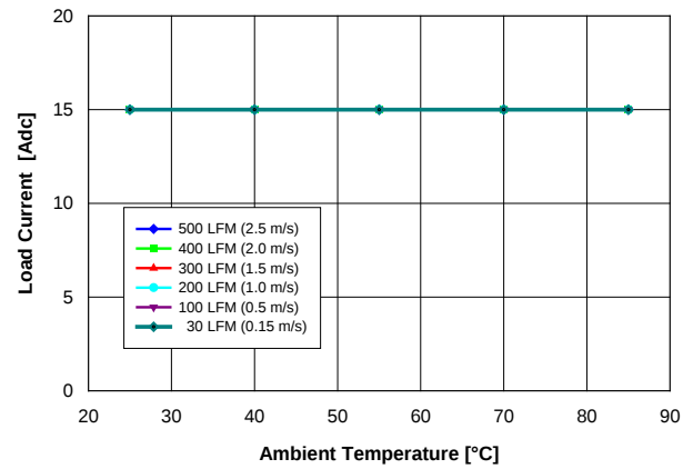
Figure 3. Power derating of SQL48T15033 converter with baseplate option and 0.25" tall horizontal-fin heatsink. (Conditions: same as Figure 1) No thermal derating required.
