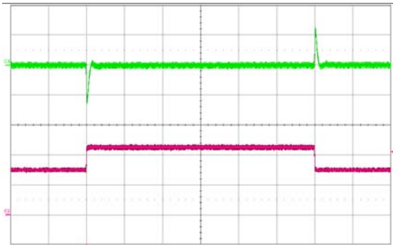
Figure 12. Output voltage response to load current step change (7.5A – 11.25A – 7.5A) at V_{in} = 48 V. Top trace: output voltage (50mV/div.) Bottom: load current (5 A/div.). Current slew rate: 1 A/ \mu s. Time scale: 200 \mu s /div. C_o = 470\mu F POS + 1 \mu F ceramic
