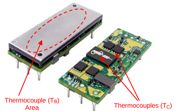
Fig. H: Locations of the thermocouples for thermal testing.
