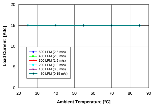
Figure 1. Available load current vs. ambient air temperature and airflow rates for SQL48T15033 converter mounted vertically with air flowing from pin 3 to pin 1, T_c temperatures \leq 120^\circ\text{C} , V_{in} = 48\text{ V} . No thermal derating required.
