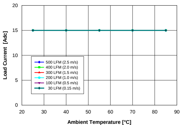
Figure 2. Power derating of SQL48T15033 converter with baseplate option. (Conditions: same as Figure 1) No thermal derating required.
