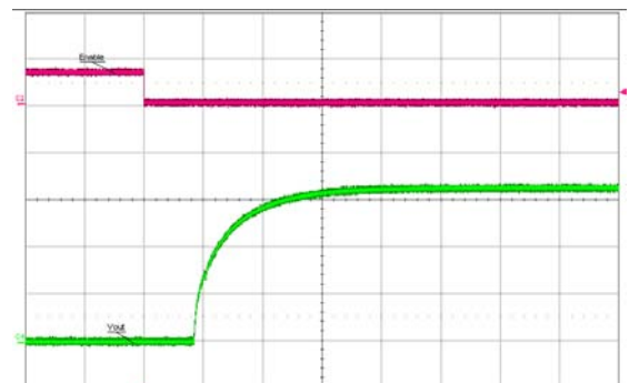
Figure 10. Turn-on waveform at full rated load current (resistive) with 10uF tant. + 1uF cer. output capacitor at V_{in} = 48\text{V} , triggered via ON/OFF pin. Top trace: ON/OFF signal (5V/div.). Bottom trace: Output voltage (1V/div.). Time scale: 2 ms/div.
