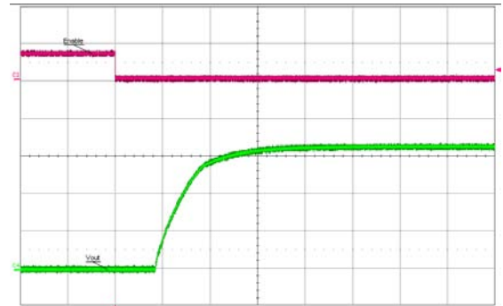
Figure 9. Turn-on waveform at full rated load current (resistive) with 7,500 uF output capacitor at V_{in}=48\text{V} , triggered via ON/OFF pin. Top trace: ON/OFF signal (5V/div.). Bottom trace: Output voltage (1V/div.). Time scale: 2 ms/div.
