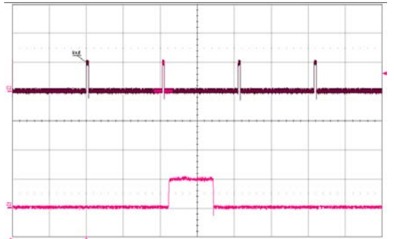
Figure 16. Load current (top trace, 20 A/div., 100 ms/div.) into a 10 m\Omega short circuit during restart, at V_{in} = 48 V. Bottom trace (20 A/div., 5 ms/div.) is an expansion of the on-time portion of the top trace.
