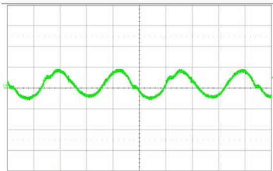
Figure 13. Output voltage ripple (20 mV/div.) at full rated load current into a resistive load with C_o = 10\mu F tantalum + 1 \mu F ceramic and V_{in} = 48 V. Time scale: 1 \mu s/div.
