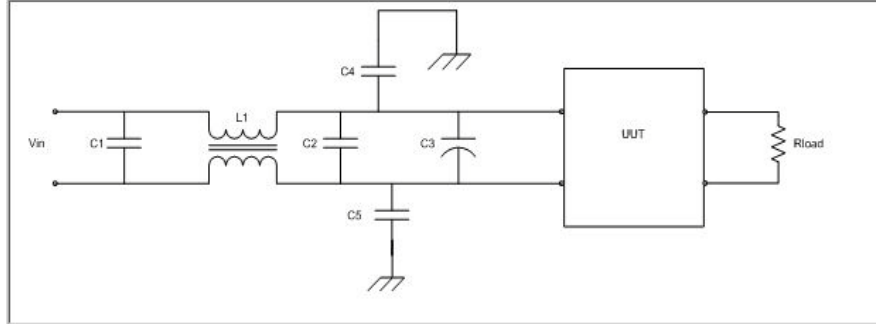
EMI filter
