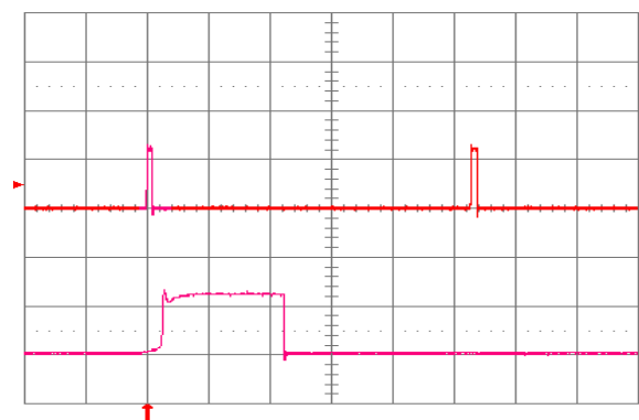
Fig. 2.0V.12: Load current (top trace, 20 A/div., 20 ms/div.) into a 10 mΩ short circuit during restart, at V_{in} = 48 V. Bottom trace (20 A/div., 1 ms/div.) is an expansion of the on-time portion of the top trace.
