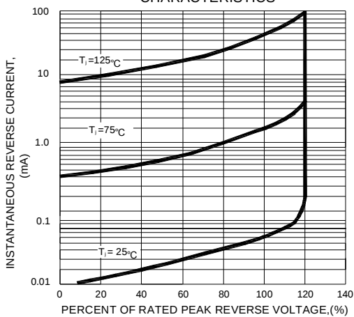
FIG.3-TYPICAL REVERSE CHARACTERISTICS
