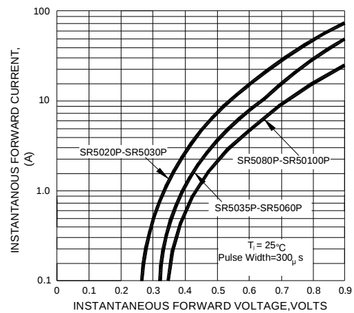
FIG.4-TYPICAL FORWARD CHARACTERISTICS
