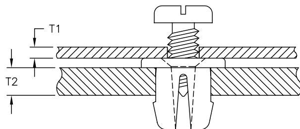
TYPICAL APPLICATION
