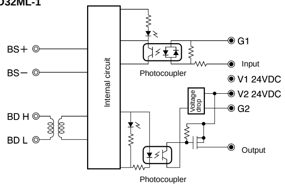
SRT2-MD32ML-1
