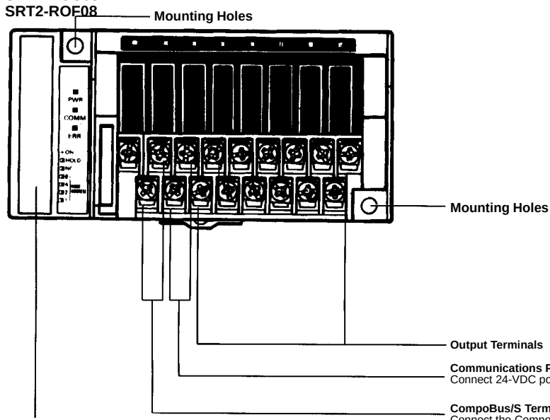
SRT2-ROC08 SRT2-ROF08
