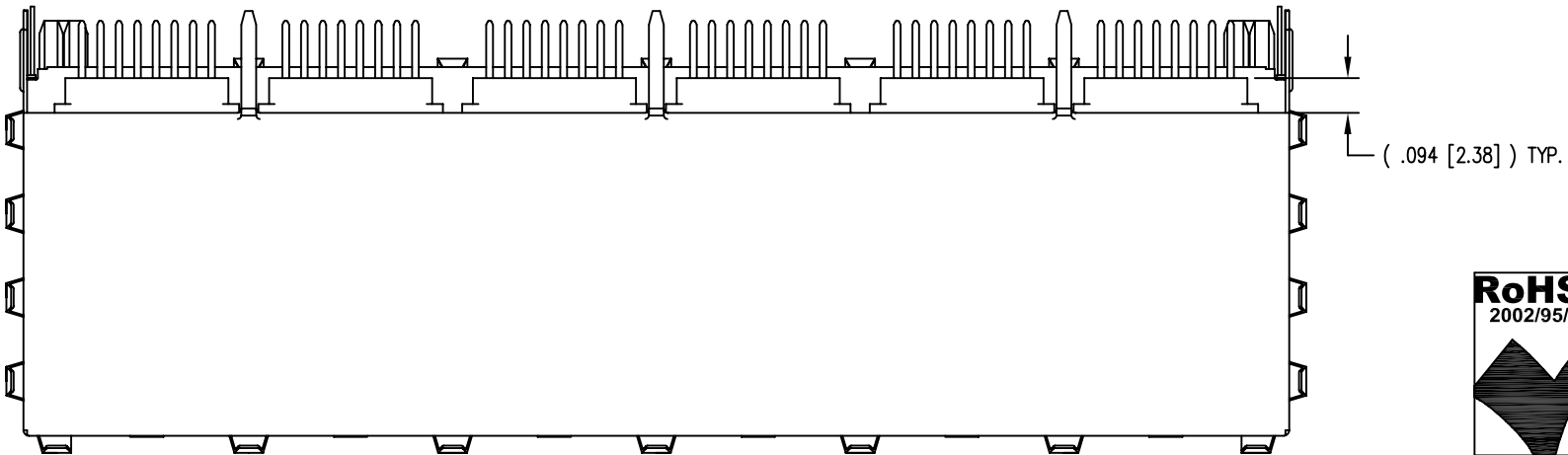
PIN DETAIL TYP. ALL PORTS
