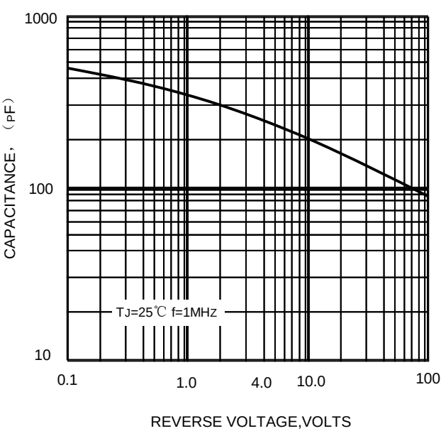
FIG.4-TYPICAL JUNCTION CAPACITANCE
