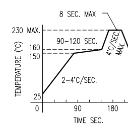
REFLOW PROFILE
