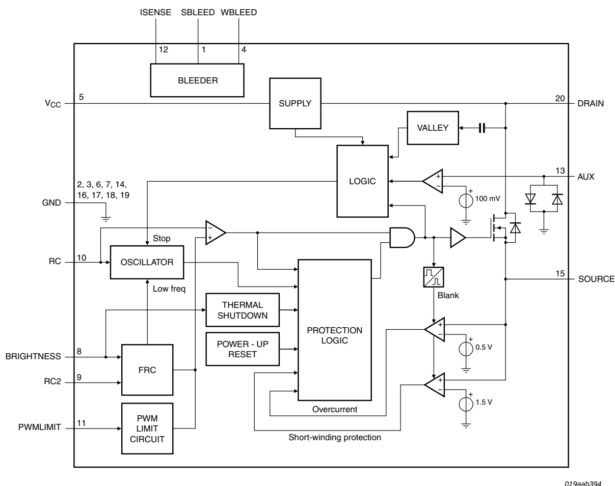
Fig 5. Block diagram SSL2102
