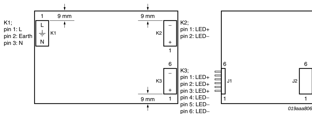
Fig 2. Board connection diagram
