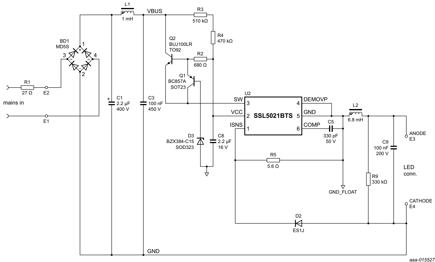
Fig 11. SSL5021BDB1267 demo board schematic diagram
