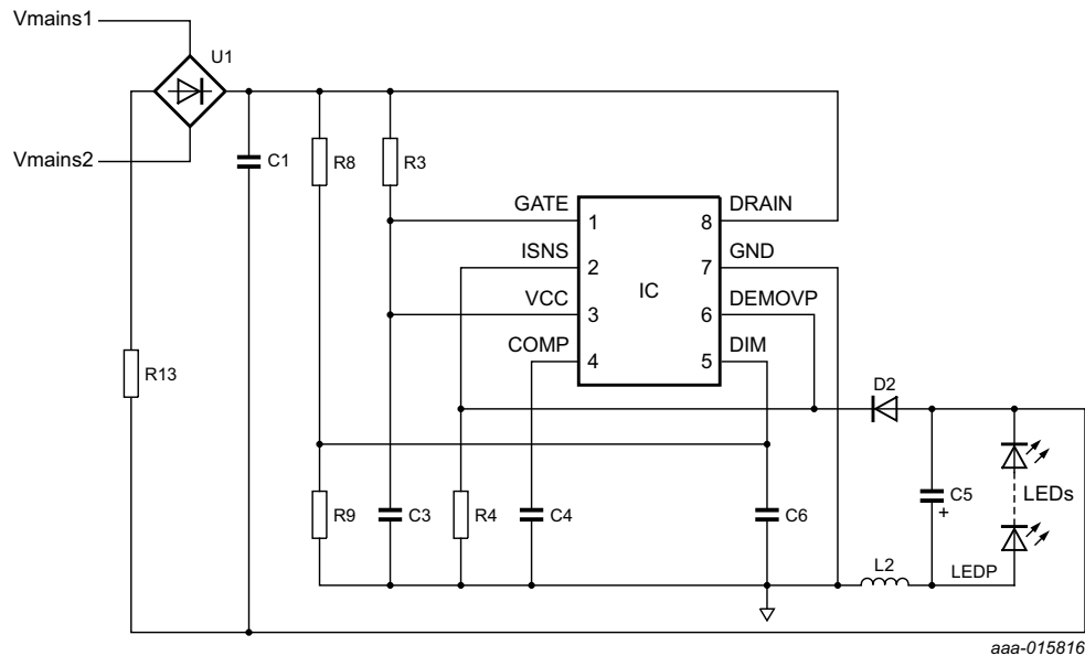
Fig 3. SSL5237BTE basic application diagram
