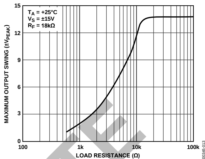
Figure 13. Maximum Output Swing vs. Load Resistance ( \text{THD} = 1\% Max)
