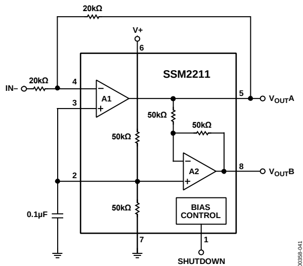
Figure 41. Simplified Schematic
