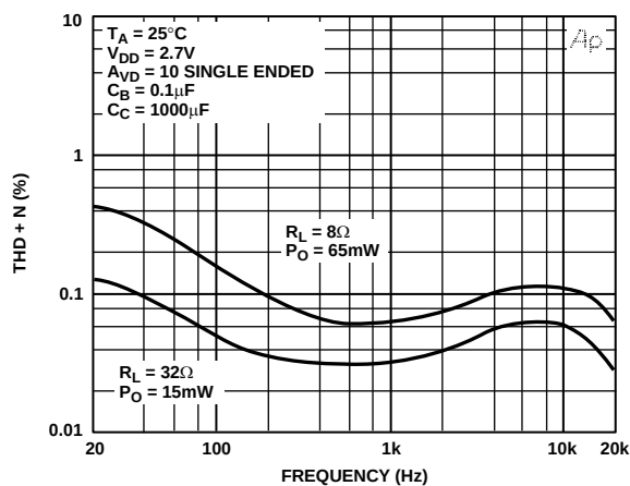
Figure 27. THD + N vs. Frequency
