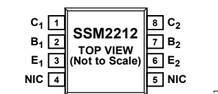
Figure 17. SOIC Pin Configuration
