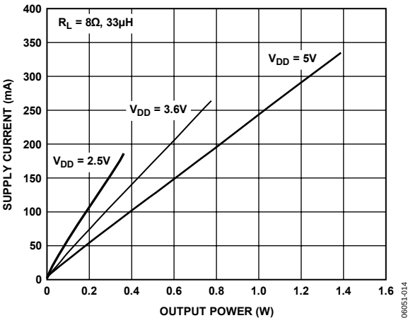
Figure 14. Output Power vs. Supply Current, One Channel
