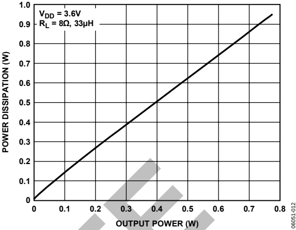
Figure 12. Power Dissipation vs. Output Power at V_{DD} = 3.6\text{V}
