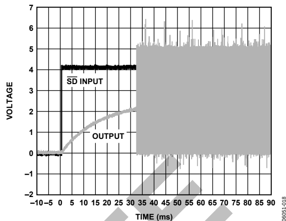
Figure 18. Turn-On Response
