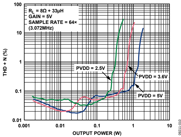
Figure 4. THD + N vs. Output Power into 8 \Omega , Gain = 5 V, f_s = 64\times
