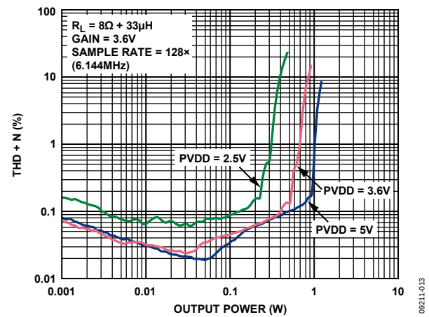
Figure 8. THD + N vs. Output Power into 8 \Omega , Gain = 3.6 V, f_s = 128\times
