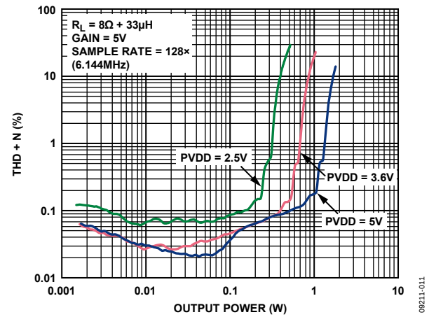
Figure 7. THD + N vs. Output Power into 8 \Omega , Gain = 5 V, f_s = 128\times
