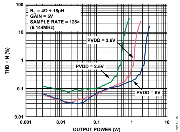
Figure 9. THD + N vs. Output Power into 4 \Omega , Gain = 5 V, f_s = 128\times
