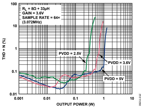
Figure 5. THD + N vs. Output Power into 8 \Omega , Gain = 3.6 V, f_s = 64\times
