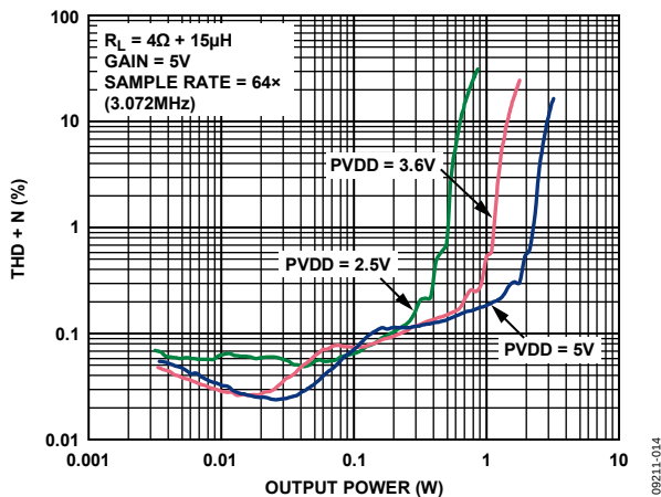
Figure 6. THD + N vs. Output Power into 4 \Omega , Gain = 5 V, f_s = 64\times
