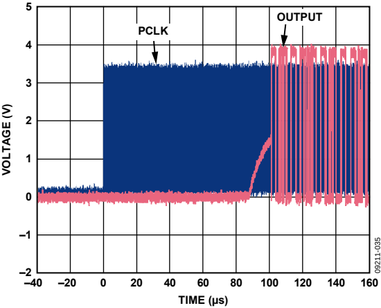
Figure 29. Turn-On Response
