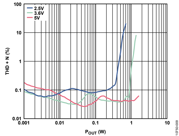
Figure 9. THD + N vs. Output Power into 4 \Omega , 3.6 V Gain Setting
