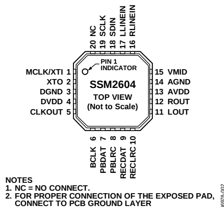
Figure 6. Pin Configuration
