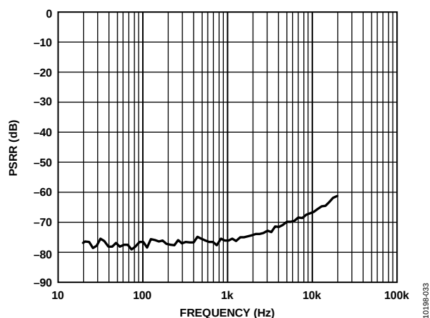
Figure 33. PSRR vs. Frequency, V_{\text{RIPPLE}} = 100 \text{ mV rms}
