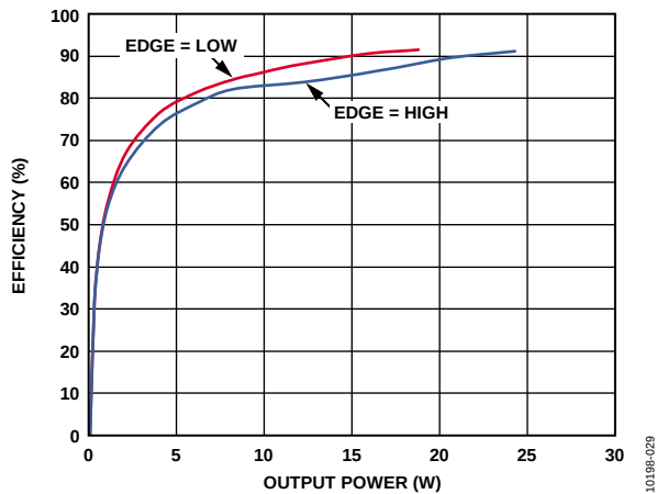
Figure 29. Efficiency vs. Output Power into 8\Omega ; PVDD = 12V ; EDGE = High , EDGE = Low
