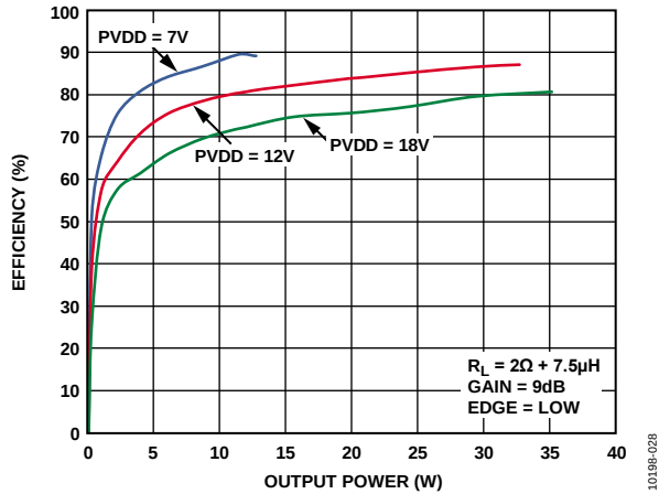
Figure 28. Efficiency vs. Output Power into 2\Omega ; Mono Mode; PVDD = 7V , PVDD = 12V , PVDD = 18V
