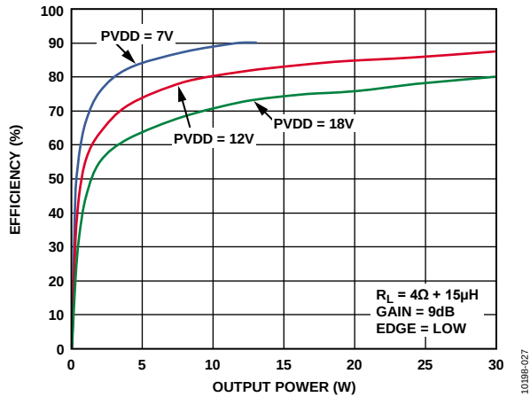
Figure 27. Efficiency vs. Output Power into 4\Omega ; PVDD = 7V , PVDD = 12V , PVDD = 18V
