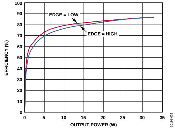
Figure 31. Efficiency vs. Output Power into 2\Omega ; Mono Mode; PVDD = 12V ; EDGE = High , EDGE = Low
