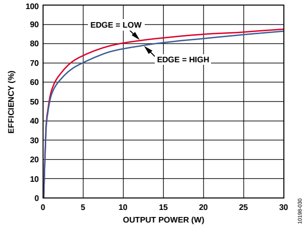
Figure 30. Efficiency vs. Output Power into 4\Omega ; PVDD = 12V ; EDGE = High , EDGE = Low
