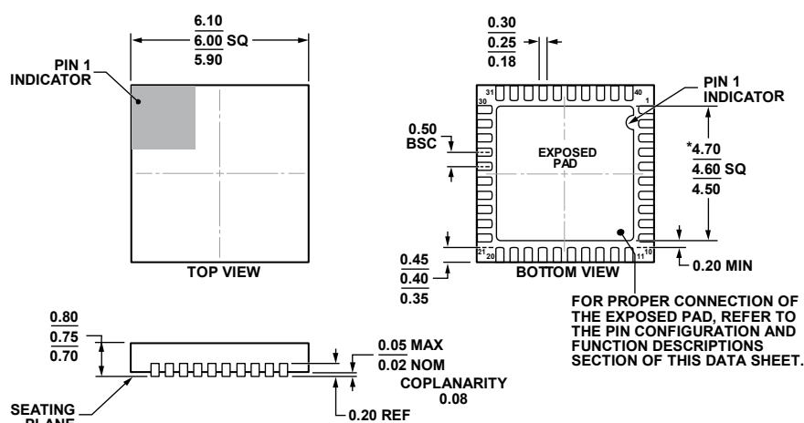
Figure 88. 40-Lead Lead Free Chip Scale Package [LFCSP] 6 mm × 6 mm Body and 0.75 mm Package Height (CP-40-7)
