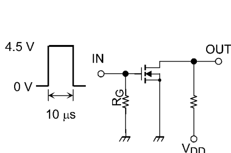
Fig. 5.3.1 Test Circuit of Switching Time
