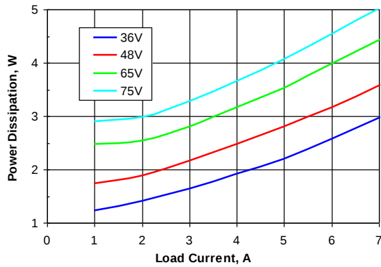
Figure 4. Power dissipation vs. load current and input voltage for SSQE48T07050 converter mounted vertically with air flowing from pin 1 to pin 3 at a rate of 300 LFM (1.5 m/s) and T_a = 25^\circ\text{C} .
