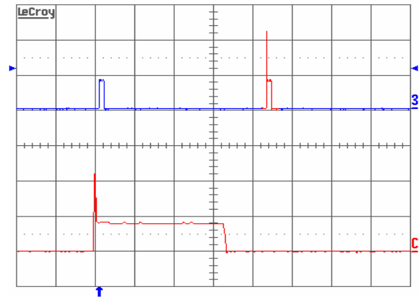
Figure 14. Load current (top trace, 5 A/div., 50 ms/div.) into a 10 \text{ m}\Omega short circuit during restart, at V_{in} = 48 \text{ V} . Bottom trace (5 A/div., 2 ms/div.) is an expansion of the on-time portion of the top trace
