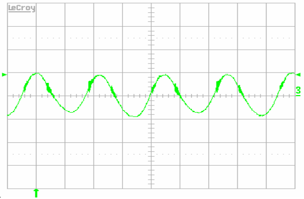
Figure 13. Input reflected ripple-current, i_c (50 mA/div.), measured at input terminals at full rated load current and V_{in} = 48 \text{ V} . Refer to Figure 11 for test setup. Time scale: 1 \mu\text{s}/\text{div} .
