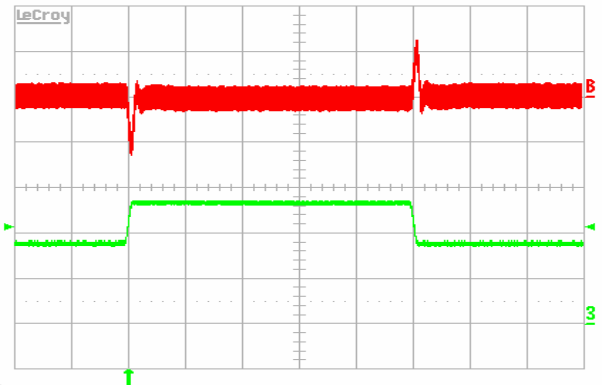
Figure 8. Output voltage response to load current step (3.5A–5.25A–3.5A) at V_{in}=48\text{ V} . Top trace: output voltage (100 mV/div.). Bottom trace: load current (2A/div.). Current slew rate: 0.1A/ \mu\text{s} . C_o=1\mu\text{F} ceramic + 10 \mu\text{F} tantalum. Time scale: 0.2ms/div.
