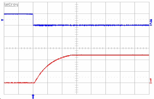
Figure 7. Turn-on transient at full rated load current (resistive) plus 3,300 \mu\text{F} at V_{in} = 48\text{ V} , triggered via ON/OFF pin. Top trace: ON/OFF signal (5 V/div.). Bottom trace: Output voltage (5 V/div.). Time scale: 2 ms/div.
