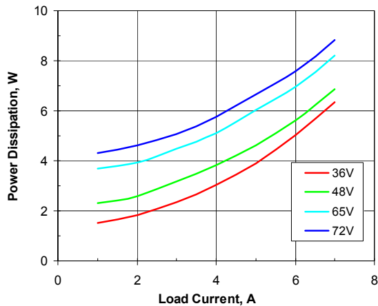
Figure 4. Power dissipation vs. load current and input voltage for SSQE48T07120 converter mounted vertically with air flowing from pin 1 to pin 3 at a rate of 300 LFM (1.5 m/s) and T_a = 25^\circ\text{C} .
