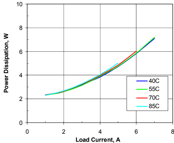
Figure 5. Power dissipation vs. load current and ambient temperature for SSQE48T07120 converter mounted vertically with V_{in} = 48\text{ V} and air flowing from pin 1 to pin 3 at a rate of 200 LFM (1.0 m/s).
