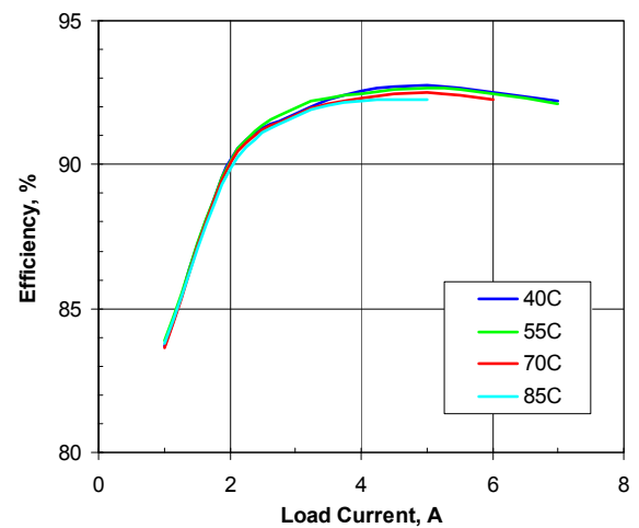
Figure 3. Efficiency vs. load current and ambient temperature for SSQE48T07120 converter mounted vertically with V_{in} = 48 V and air flowing from pin 1 to pin 3 at a rate of 200 LFM (1.0 m/s).
