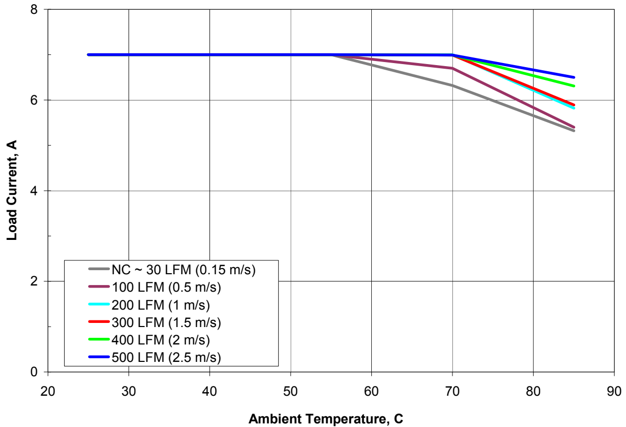
Figure 1. Available load current vs. ambient air temperature and airflow rates for SSQE48T07120 converter mounted vertically with air flowing from pin 1 to pin 3, V_{in} = 48 V. Note: NC – Natural convection
