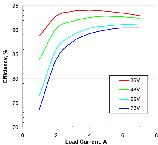
Figure 2. Efficiency vs. load current and input voltage for SSQE48T07120 converter mounted vertically with air flowing from pin 1 to pin 3 at a rate of 300 LFM (1.5 m/s) and T_a = 25^\circ\text{C} .
