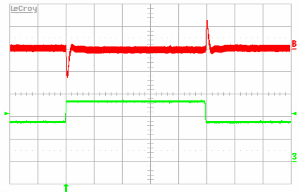
Figure 9. Output voltage response to load current step (3.5A–5.25A–3.5A) at V_{in}=48\text{ V} . Top trace: output voltage (100 mV/div.). Bottom trace: load current (2A/div.). Current slew rate: 1A/ \mu\text{s} . C_o= 100\mu\text{F} Tantalum + 1 \mu\text{F} ceramic. Time scale: 0.2 ms/div.
