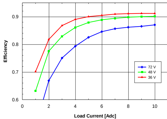
Figure 2. Efficiency vs. load current and input voltage for SSQE48T10033 converter mounted vertically with air flowing from pin 1 to pin 3 at a rate of 300 LFM (1.5 m/s) and T_a = 25^\circ\text{C} .
