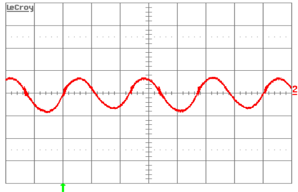
Figure 13. Input reflected ripple-current, i_c (100 mA/div.), measured at input terminals at full rated load current and V_{in} = 48 V. Refer to Figure 11 for test setup. Time scale: 1 \mu s/div.
