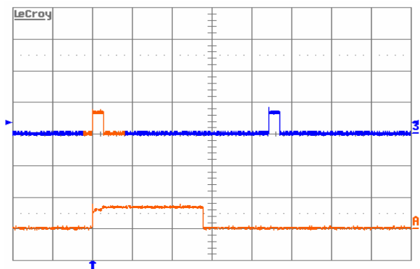
Figure 15. Load current (top trace, 20 A/div., 50 ms/div.) into a 10 m \Omega short circuit during restart, at V_{in} = 48 V. Bottom trace (20 A/div., 5 ms/div.) is an expansion of the on-time portion of the top trace
