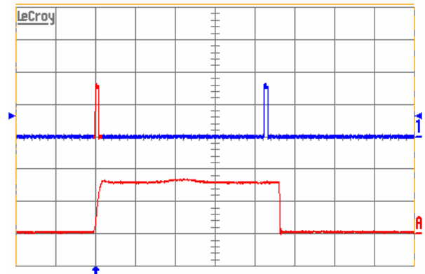
Figure 15. Load current (top trace, 10 \text{ A}/\text{div.} , 50 \text{ ms}/\text{div.} ) into a 10 \text{ m}\Omega short circuit during restart, at V_{in} = 48 \text{ V} . Bottom trace ( 10 \text{ A}/\text{div.} , 1.0 \text{ ms}/\text{div.} ) is an expansion of the on-time portion of the top trace
