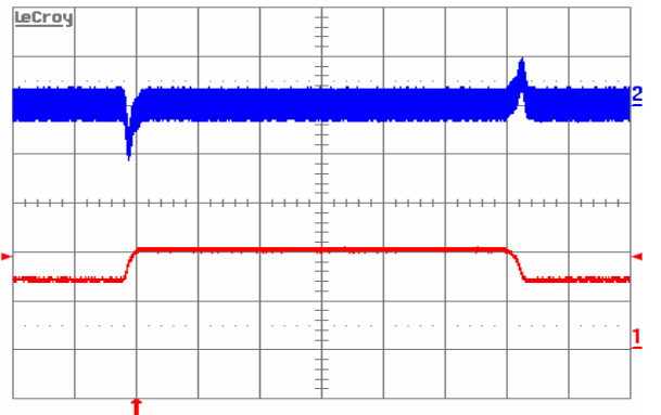
Figure 8. Output voltage response to load current step-change (6.5A-9.75A-6.5A) at V_{in}=48\text{V} . Top trace: output voltage (100 mV/div.). Bottom trace: load current (5A/div.). Current slew rate: 0.1A/ \mu\text{s} . C_o=1\mu\text{F} ceramic + 10 \mu\text{F} tantalum. Time scale: 0.2ms/div.
