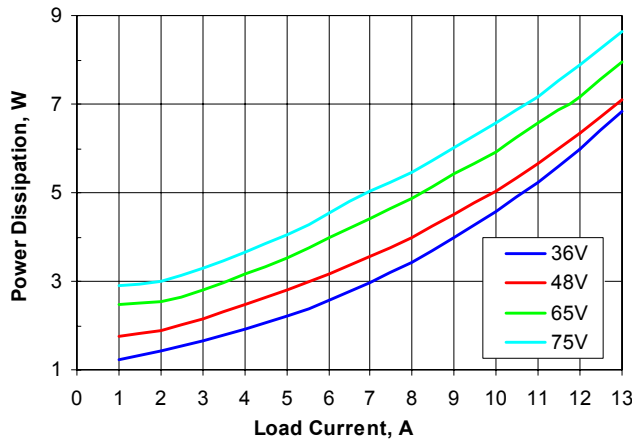
Figure 4. Power dissipation vs. load current and input voltage for SSQE48T13050 converter mounted vertically with air flowing from pin 1 to pin 3 at a rate of 300 LFM (1.5 m/s) and T_a = 25^\circ\text{C} .
