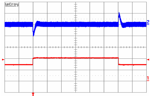
Figure 9. Output voltage response to load current step-change (6.5A-9.75A-6.5A) at V_{in}=48\text{V} . Top trace: output voltage (100 mV/div.). Bottom trace: load current (5A/div.). Current slew rate: 5A/ \mu\text{s} . C_o=470\mu\text{F} POS + 1 \mu\text{F} ceramic. Time scale: 0.2 ms/div.
