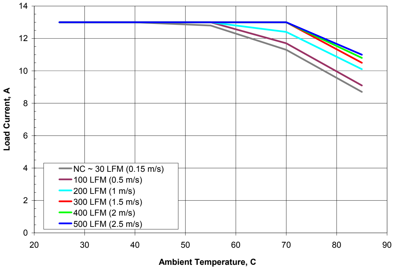
Figure 1. Available load current vs. ambient air temperature and airflow rates for SSQE48T13050 converter mounted vertically with air flowing from pin 1 to pin 3, V_{in} = 48\text{ V} . Note: NC – Natural convection
