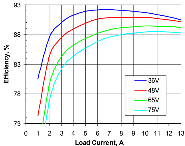
Figure 2. Efficiency vs. load current and input voltage for SSQE48T13050 converter mounted vertically with air flowing from pin 1 to pin 3 at a rate of 300 LFM (1.5 m/s) and T_a = 25^\circ\text{C} .
