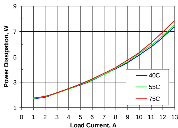
Figure 5. Power dissipation vs. load current and ambient temperature for SSQE48T13050 converter mounted vertically with V_{in} = 48\text{ V} and air flowing from pin 1 to pin 3 at a rate of 200 LFM (1.0 m/s).
