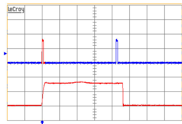
Figure 15. Load current (top trace, 10 A/div., 50 ms/div.) into a 10 m \Omega short circuit during restart, at V_{in} = 48 V. Bottom trace (10 A/div., 1.0 ms/div.) is an expansion of the on-time portion of the top trace.
