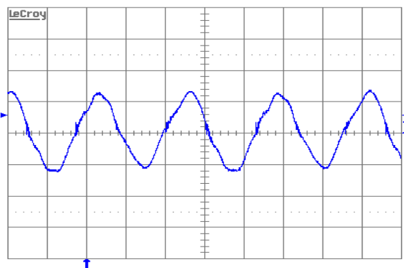
Figure 10. Output voltage ripple (20 mV/div.) at full rated load current into a resistive load with C_o = 10\mu\text{F} tantalum + 1 \mu\text{F} ceramic and V_{\text{in}} = 48\text{ V} . Time scale: 1 \mu\text{s} /div.
