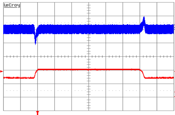
Figure 8. Output voltage response to load current step-change (6.5A–9.75A–6.5A) at V_{\text{in}}=48\text{V} . Top trace: output voltage (100 mV/div.). Bottom trace: load current (5A/div.). Current slew rate: 0.1A/ \mu\text{s} . C_o=1\mu\text{F} ceramic + 10 \mu\text{F} tantalum. Time scale: 0.2ms/div.
