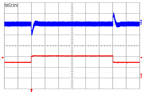
Figure 9. Output voltage response to load current step-change (6.5A–9.75A–6.5A) at V_{\text{in}}=48\text{V} . Top trace: output voltage (100 mV/div.). Bottom trace: load current (5A/div.). Current slew rate: 5A/ \mu\text{s} . C_o=470\mu\text{F} POS + 1 \mu\text{F} ceramic. Time scale: 0.2 ms/div.
