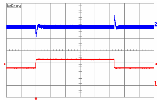
Figure 9. Output voltage response to load current step-change (7.5A–10.25A–7.5A) at V_{in}=48\text{V} . Top trace: output voltage (100 mV/div.). Bottom trace: load current (5A/div.). Current slew rate: 5A/ \mu\text{s} . C_o=470\mu\text{F} POS + 1 \mu\text{F} ceramic. Time scale: 0.2 ms/div.
