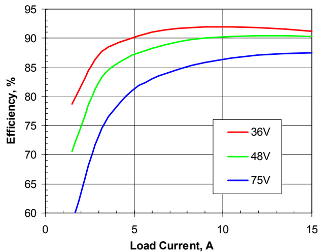
Figure 2. Efficiency vs. load current and input voltage for SSQE48T15033 converter mounted vertically with air flowing from pin 1 to pin 3 at a rate of 300 LFM (1.5 m/s) and Ta=25°C.
