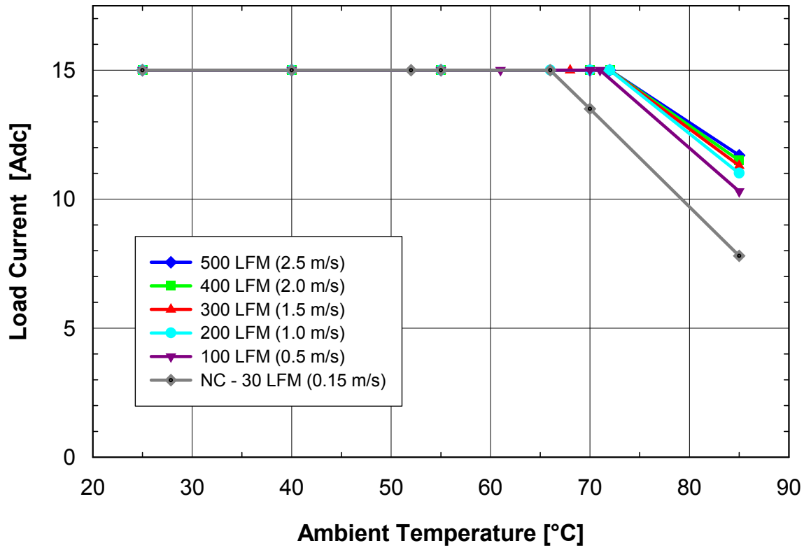
Figure 1. Available load current vs. ambient air temperature and airflow rates for SSQE48T15033 converter mounted vertically with air flowing from pin 1 to pin 3, Vin = 48 V. Note: NC – Natural convection
