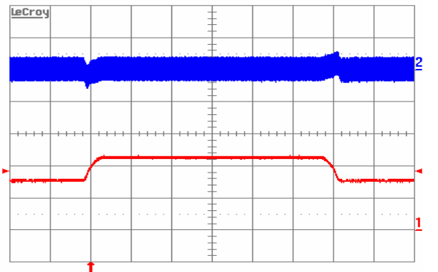
Figure 8. Output voltage response to load current step-change (7.5A–10.25A–7.5A) at V_{in}=48\text{V} . Top trace: output voltage (100 mV/div.). Bottom trace: load current (5A/div.). Current slew rate: 0.1A/ \mu\text{s} . C_o=1\mu\text{F} ceramic + 10 \mu\text{F} tantalum. Time scale: 0.2ms/div.
