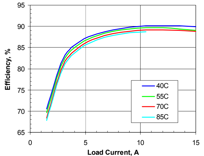
Figure 3. Efficiency vs. load current and ambient temperature for SSQE48T15033 converter mounted vertically with Vin=48V and air flowing from pin 1 to pin 3 at a rate of 200LFM (1.0m/s).
