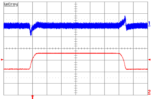
Figure 8. Output voltage response to load current step (12.5A–18.75A–12.5A) at V_{in}=48\text{ V} . Top trace: output voltage (50 mV/div.). Bottom trace: load current (5A/div.). Current slew rate: 0.1A/ \mu\text{s} . C_o=1\mu\text{F} ceramic + 10 \mu\text{F} tantalum. Time scale: 0.2ms/div.
