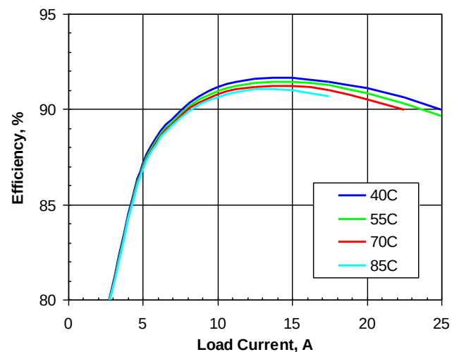
Figure 3. Efficiency vs. load current and ambient temperature for SSQE48T25033 converter mounted vertically with V_{in} = 48\text{ V} and air flowing from pin 1 to pin 3 at a rate of 200LFM (1.0m/s).
