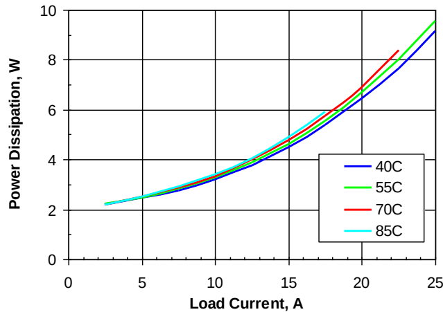
Figure 5. Power dissipation vs. load current and ambient temperature for SSQE48T25033 converter mounted vertically with V_{in} = 48\text{ V} and air flowing from pin 1 to pin 3 at a rate of 200 LFM (1.0 m/s).
