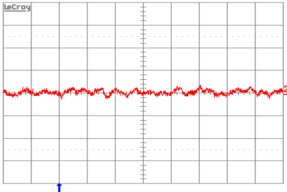
Figure 12. Input reflected-ripple current, i_s (10 mA/div.), measured through 10 \mu\text{H} at the source at full
