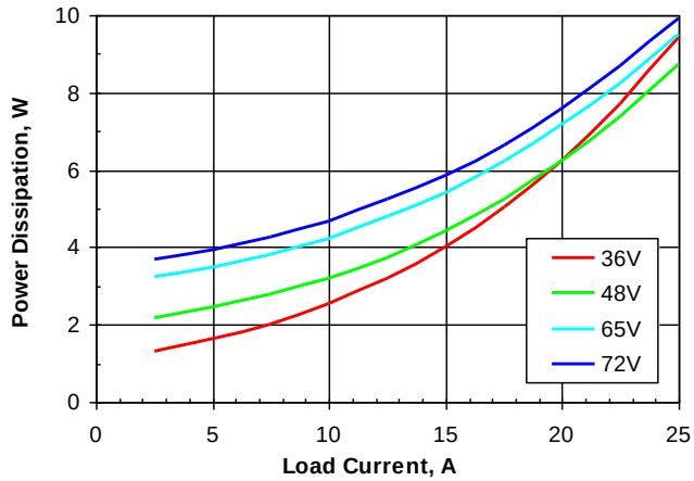
Figure 4. Power dissipation vs. load current and input voltage for SSQE48T25033 converter mounted vertically with air flowing from pin 1 to pin 3 at a rate of 300 LFM (1.5 m/s) and T_a = 25^\circ\text{C} .
