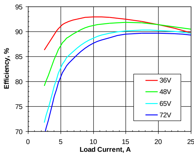
Figure 2. Efficiency vs. load current and input voltage for SSQE48T25033 converter mounted vertically with air flowing from pin 1 to pin 3 at a rate of 300 LFM (1.5 m/s) and T_a = 25^\circ\text{C} .
