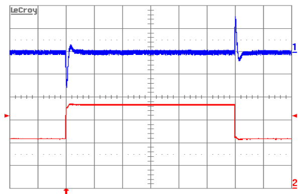
Figure 9. Output voltage response to load current step (12.5A–18.75A–12.5A) at V_{in}=48\text{ V} . Top trace: output voltage (100 mV/div.). Bottom trace: load current (5A/div.). Current slew rate: 5A/ \mu\text{s} . C_o=470\mu\text{F} POS + 1 \mu\text{F} ceramic. Time scale: 0.2 ms/div.
