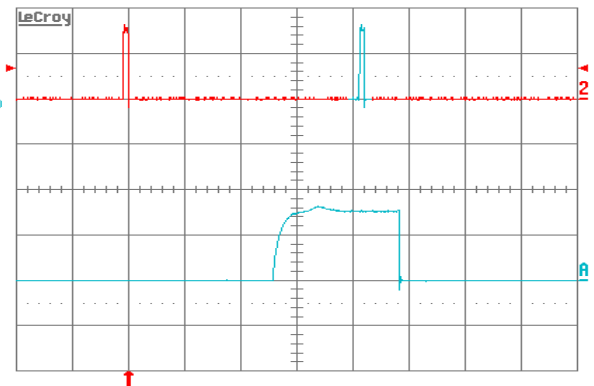
Figure 14. Load current (top trace, 20 A/div., 50 ms/div.) into a 10 \text{ m}\Omega short circuit during restart, at V_{in} = 48 \text{ V} . Bottom trace (20 A/div., 2 ms/div.) is an expansion of the on-time portion of the top trace
