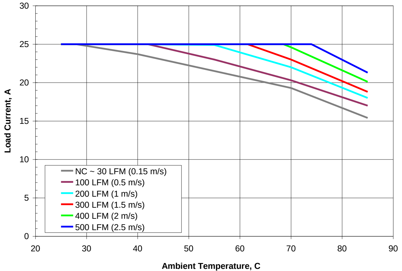
Figure 1. Available load current vs. ambient air temperature and airflow rates for SSQE48T25033 converter mounted vertically with air flowing from pin 1 to pin 3, V_{in} = 48\text{ V} . Note: NC – Natural convection
