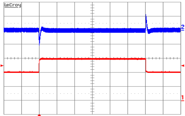
Figure 9: Output voltage response to load current step-change (10A–15A–10A) at V_{in}=48\text{V} . Top trace: output voltage (100 mV/div.). Bottom trace: load current (5A/div.). Current slew rate: 5A/ \mu\text{s} . C_o= 470\mu\text{F} POS + 1 \mu\text{F} ceramic. Time scale: 0.2 mS/div.
