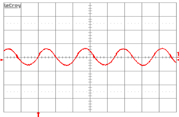
Figure 13: Input reflected-ripple-current, i_c (200 mA/div.), through 10 \mu\text{H} measured at input terminals at full rated load current and V_{in} = 48 \text{ V} . Refer to Figure 11 for test setup. Time scale: 1 \mu\text{s}/\text{div} .
