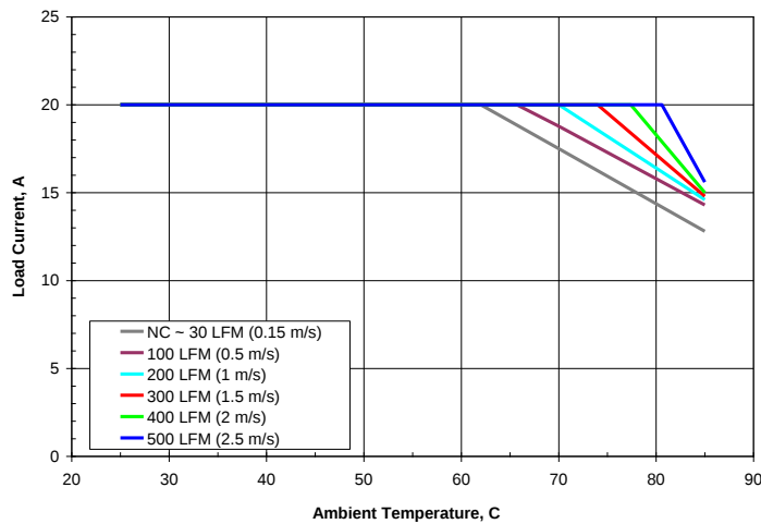
Figure 1: Available load current vs. ambient air temperature and airflow rates for SSQE48T20033 converter mounted vertically with air flowing from pin 1 to pin 3, V_{in} = 48\text{ V} . Note: NC – Natural convection
