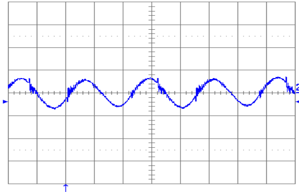
Figure 10: Output voltage ripple (50 mV/div.) at full rated load current into a resistive load with C_o = 10 \mu\text{F} tantalum + 1 \mu\text{F} ceramic and V_{in} = 48 \text{ V} . Time scale: 1 \mu\text{s}/\text{div} .
