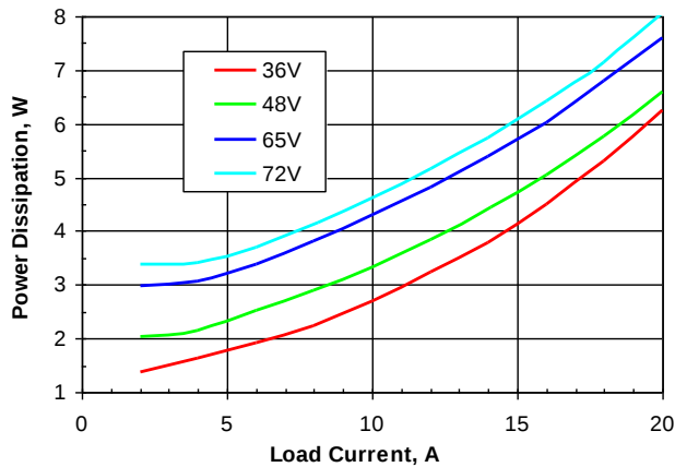
Figure 4: Power dissipation vs. load current and input voltage for SSQE48T20033 converter mounted vertically with air flowing from pin 1 to pin 3 at a rate of 300 LFM (1.5 m/s) and T_a = 25^\circ\text{C} .
