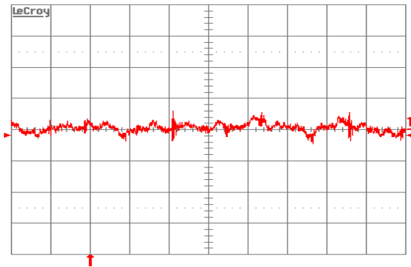
Figure 12: Input reflected-ripple current, i_s (10 mA/div.), measured \mu\text{H} at the source at full rated load current and V_{in} = 48 \text{ V} . Refer to Figure 11 or test setup. Time scale: 1 \mu\text{s}/\text{div} .
