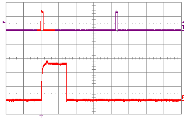
Figure 15: Load current (top trace, 20 \text{ A}/\text{div} ., 50 \text{ mS}/\text{div} .) into a 10 \text{ m}\Omega short circuit during restart, at V_{in} = 48 \text{ V} . Bottom trace ( 10 \text{ A}/\text{div} ., 5 \text{ mS}/\text{div} .) is an expansion of the on-time portion of the top trace.
