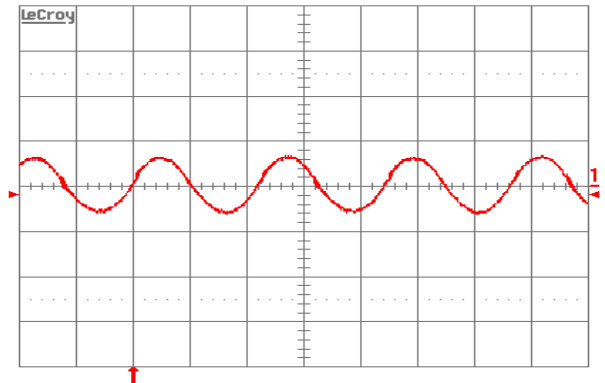
Figure 13. Input reflected ripple-current, i_c (200 mA/div.), measured at input terminals at full rated load current and V_{in} = 48\ \text{V} . Refer to Figure 11 for test setup. Time scale: 1\ \mu\text{s}/\text{div} .
