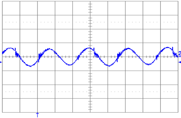
Figure 10. Output voltage ripple (50 mV/div.) at full rated load current into a resistive load with C_o = 10\ \mu\text{F} tantalum + 1\ \mu\text{F} ceramic and V_{in} = 48\ \text{V} . Time scale: 1\ \mu\text{s}/\text{div} .
