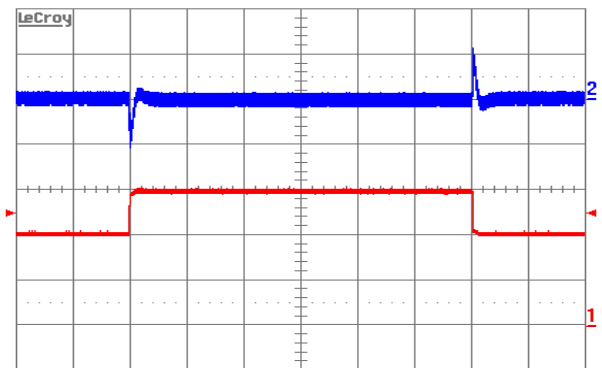
Figure 9. Output voltage response to load current step-change (10A–15A–10A) at V_{in}=48\text{V} . Top trace: output voltage (100 mV/div.). Bottom trace: load current (5A/div.). Current slew rate: 5\text{ A}/\mu\text{s} . C_o= 470\mu\text{F} POS + 1\mu\text{F} ceramic. Time scale: 0.2 mS/div.
