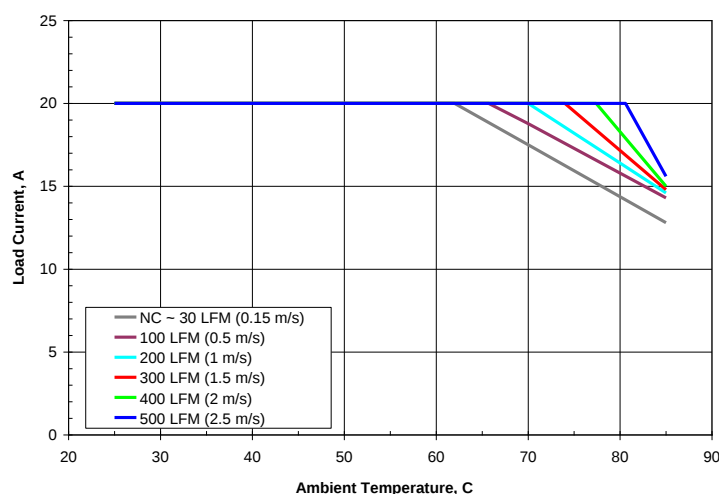
Figure 1. Available load current vs. ambient air temperature and airflow rates for SSQE48T20033 converter mounted vertically with air flowing from pin 1 to pin 3, V_{in} = 48\text{V} . Note: NC – Natural convection
