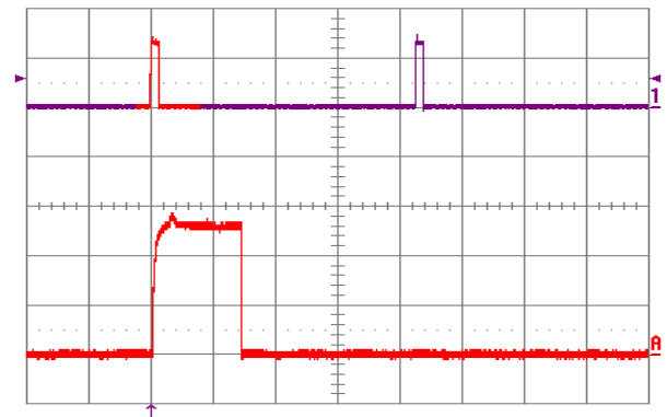
Figure 15. Load current (top trace, 20 A/div., 50 mS/div.) into a 10\ \text{m}\Omega short circuit during restart, at V_{in} = 48\ \text{V} . Bottom trace (10 A/div., 5 mS/div.) is an expansion of the on-time portion of the top trace
