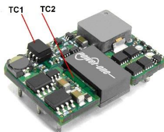
Fig. H: Locations of the thermocouple for thermal testing.
