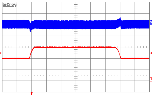
Figure 8. Output voltage response to load current step-change (10A–15A–10A) at V_{in}=48\text{V} . Top trace: output voltage (100 mV/div.). Bottom trace: load current (5A/div.). Current slew rate: 0.1\text{ A}/\mu\text{s} . C_o=1\mu\text{F} ceramic + 10\mu\text{F} tantalum. Time scale: 0.2mS/div.
