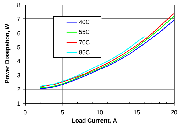
Figure 5. Power dissipation vs. load current and ambient temperature for SSQE48T20033 converter mounted vertically with V_{in} = 48\text{ V} and air flowing from pin 1 to pin 3 at a rate of 200 LFM (1.0 m/s).
