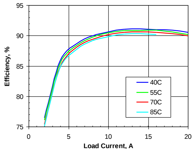
Figure 3. Efficiency vs. load current and ambient temperature for SSQE48T20033 converter mounted vertically with V_{in} = 48\text{V} and air flowing from pin 1 to pin 3 at a rate of 200 LFM (1.0 m/s).
