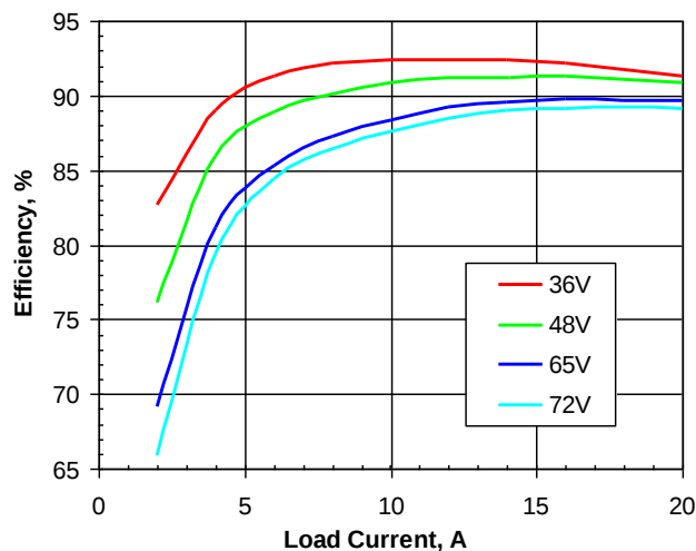
Figure 2. Efficiency vs. load current and input voltage for SSQE48T20033 converter mounted vertically with air flowing from pin 1 to pin 3 at a rate of 300 LFM (1.5 m/s) and T_a = 25^\circ\text{C} .
