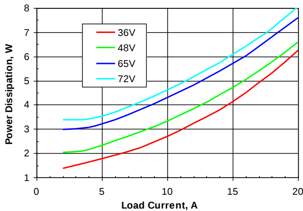
Figure 4. Power dissipation vs. load current and input voltage for SSQE48T20033 converter mounted vertically with air flowing from pin 1 to pin 3 at a rate of 300 LFM (1.5 m/s) and T_a = 25\text{ }^{\circ}\text{C} .
