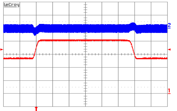
Figure 8. Output voltage response to load current step-change (12.5A-18.75A-12.5A) at V_{in}=48\text{ V} . Top trace: output voltage (100mV/div.). Bottom trace: load current (5A/div.). Current slew rate: 0.1A/ \mu\text{s} . C_o=1\mu\text{F cer}+10\mu\text{F tant} . Time scale: 0.2ms/div.
