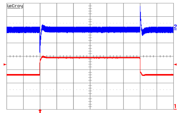
Figure 9. Output voltage response to load current step-change (12.5A-18.75A-12.5A) at V_{in}=48\text{ V} . Top trace: output voltage (100 mV/div.). Bottom trace: load current (5A/div.). Current slew rate: 5A/ \mu\text{s} . C_o=470\mu\text{F POS}+1\mu\text{F cer} . Time scale: 0.2ms/div.
