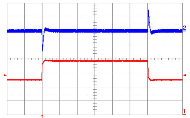
Figure 9. Output voltage response to load current step-change (12.5A–18.75A–12.5A) at V_{in}=48\text{V} . Top trace: output voltage (100 mV/div.). Bottom trace: load current (5A/div.). Current slew rate: 5A/ \mu\text{s} . C_o=470\mu\text{F POS}+1\mu\text{F cer} . Time scale: 0.2ms/div.
