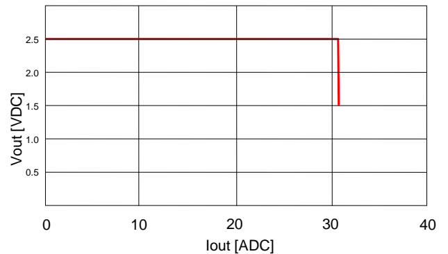
Figure 14. Output voltage vs. load current showing current limit point and converter shutdown point. Input voltage has almost no effect on current limit characteristic.
