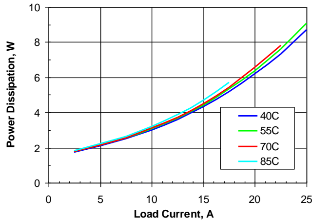
Figure 5. Power dissipation vs. load current and ambient temperature for SSQE48T25025 converter mounted vertically with V_{in} = 48\text{ V} and air flowing from pin 1 to pin 3at a rate of 200 LFM (1.0 m/s).
