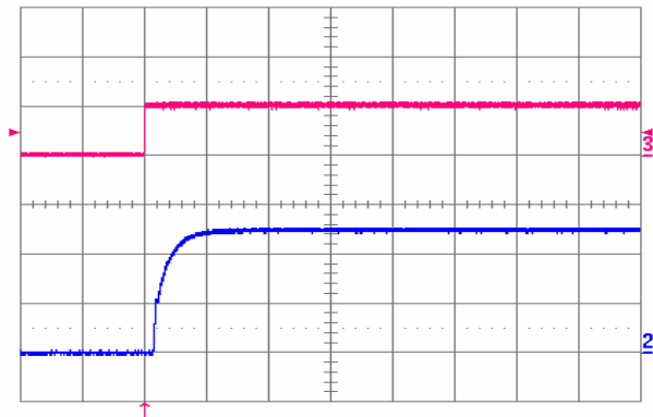
Figure 6. Turn-on transient at full rated load current (resistive) with C_o=1\mu\text{F cer}+10\mu\text{F tant} at V_{in} = 48\text{ V} , triggered via ON/OFF pin. Top trace: ON/OFF signal (5 V/div.). Bottom trace: Output voltage (1.0 V/div.). Time scale: 5 ms/div.
