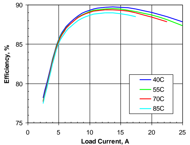
Figure 3. Efficiency vs. load current and ambient temperature for SSQE48T25025 converter mounted vertically with Vin=48V and air flowing from pin 1 to pin 3 at a rate of 200LFM (1.0m/s).
