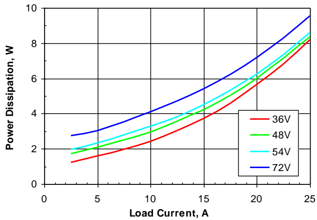
Figure 4. Power dissipation vs. load current and input voltage for SSQE48T25025 converter mounted vertically with air flowing from pin 1 to pin 3at a rate of 300 LFM (1.5 m/s) and T_a = 25^\circ\text{C} .
