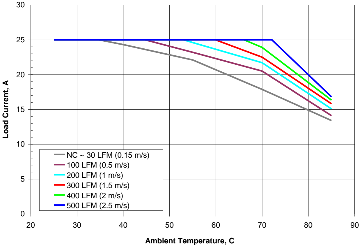
Figure 1. Available load current vs. ambient air temperature and airflow rates for SSQE48T25025 converter mounted vertically with air flowing from pin 1 to pin 3, Vin = 48 V. Note: NC – Natural convection
