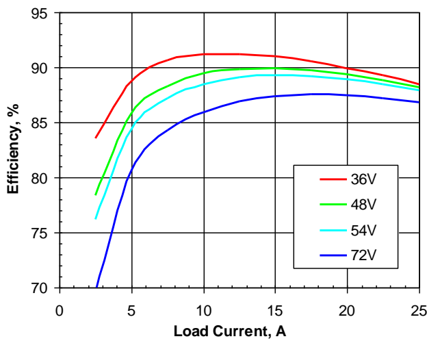
Figure 2. Efficiency vs. load current and input voltage for SSQE48T25025 converter mounted vertically with air flowing from pin 1 to pin 3 at a rate of 300 LFM (1.5 m/s) and Ta=25°C.
