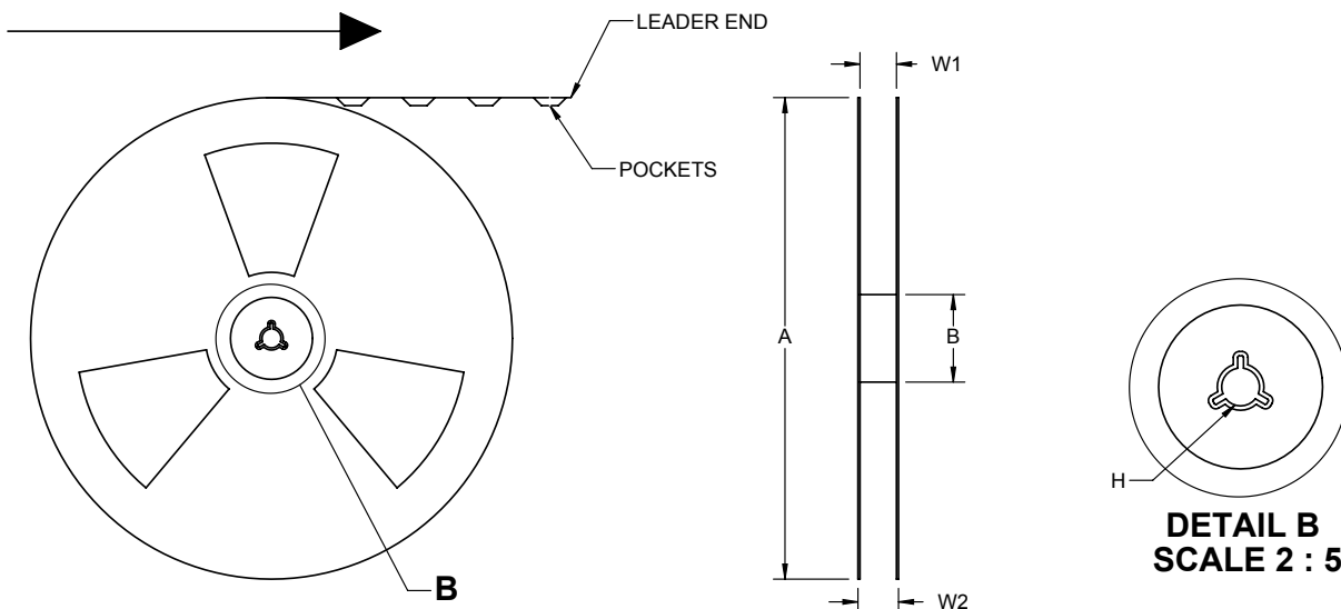
UNREELING DIRECTION
