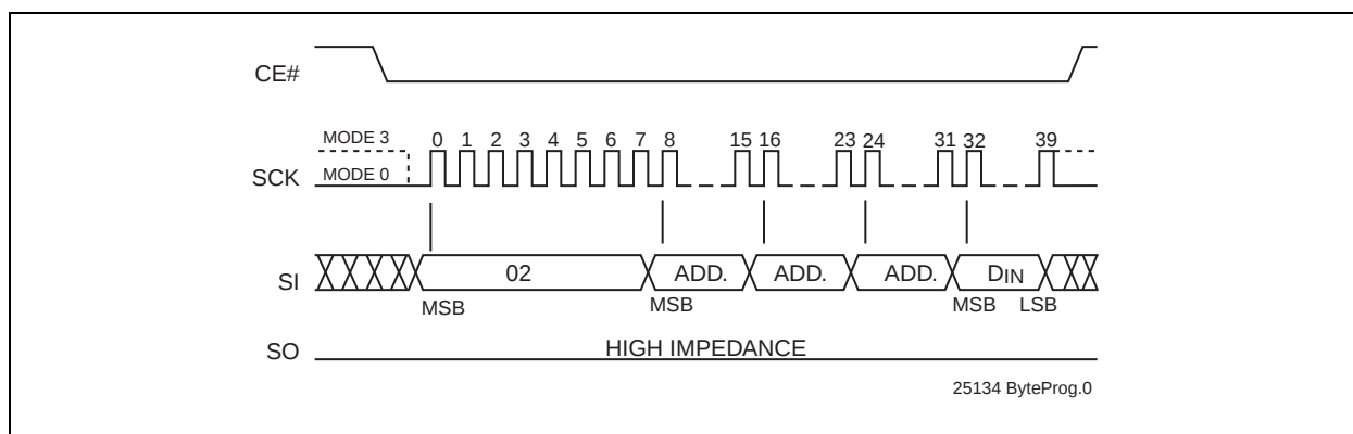
FIGURE 4-5: BYTE-PROGRAM SEQUENCE
