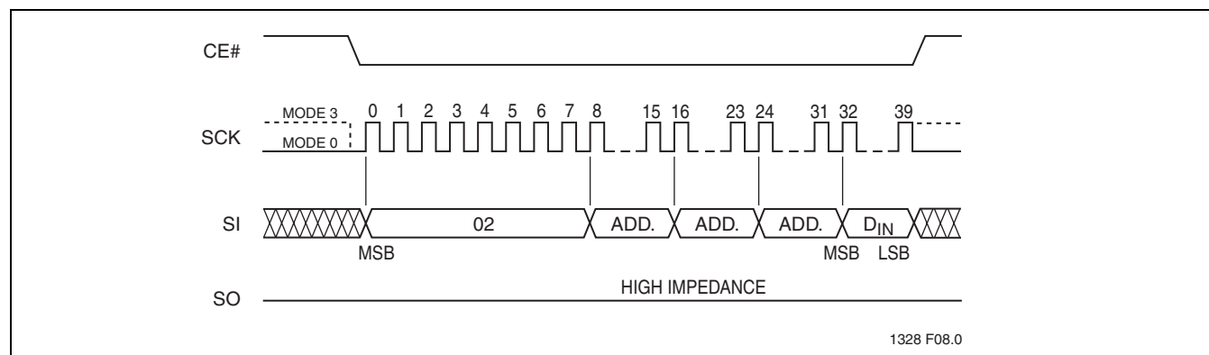
FIGURE 8: Byte-Program Sequence
