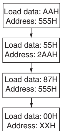
FIGURE 6-30: IRREVERSIBLE BLOCK LOCK IN MAIN ARRAY
