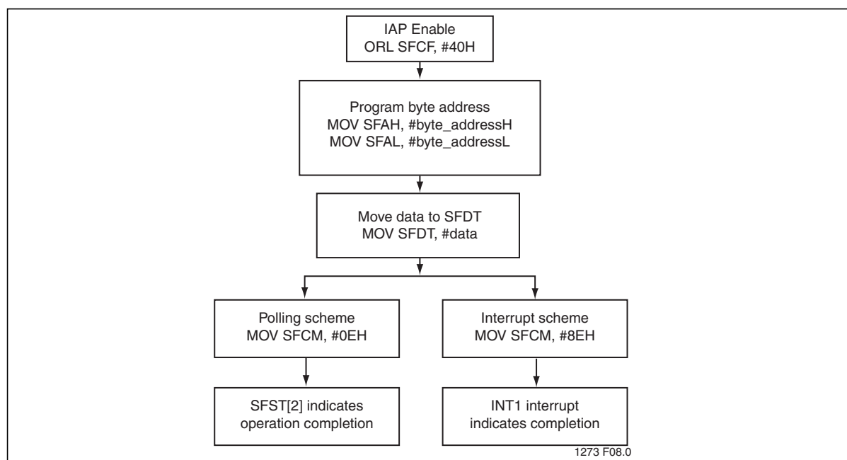
Figure 12: Byte Program
