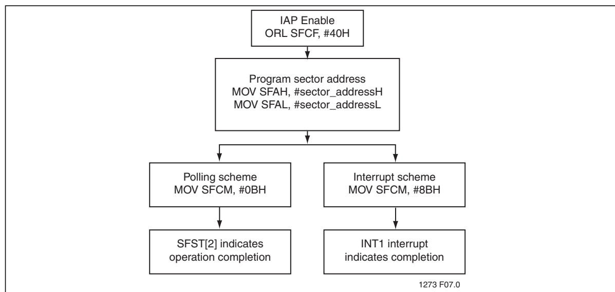
Figure 11: Sector Erase
