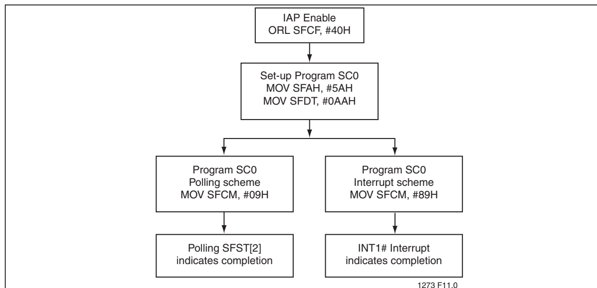
Figure 15: Prog-SC0
