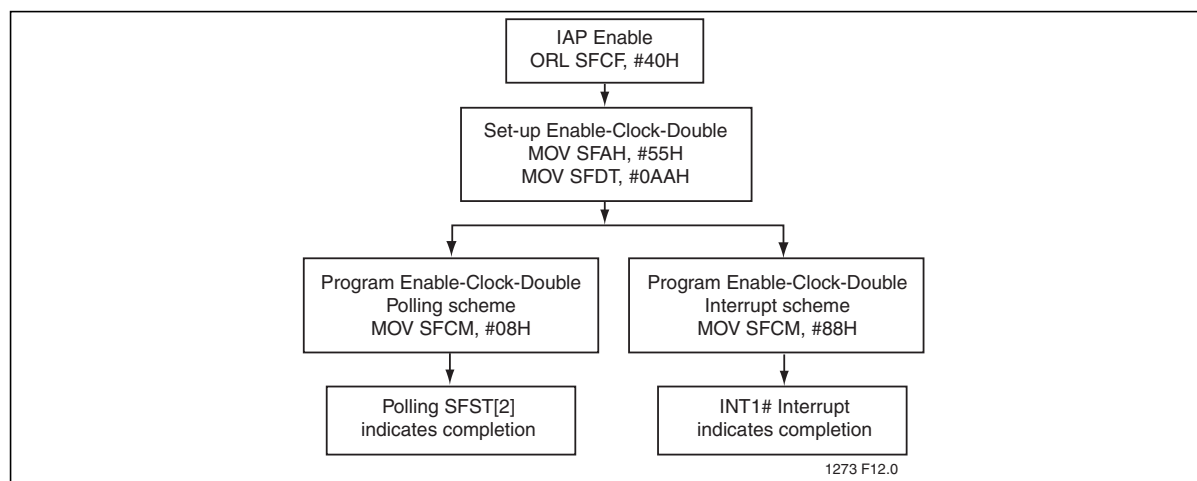
Figure 16: Enable-Clock-Double
