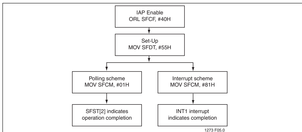
Figure 9: Chip Erase
