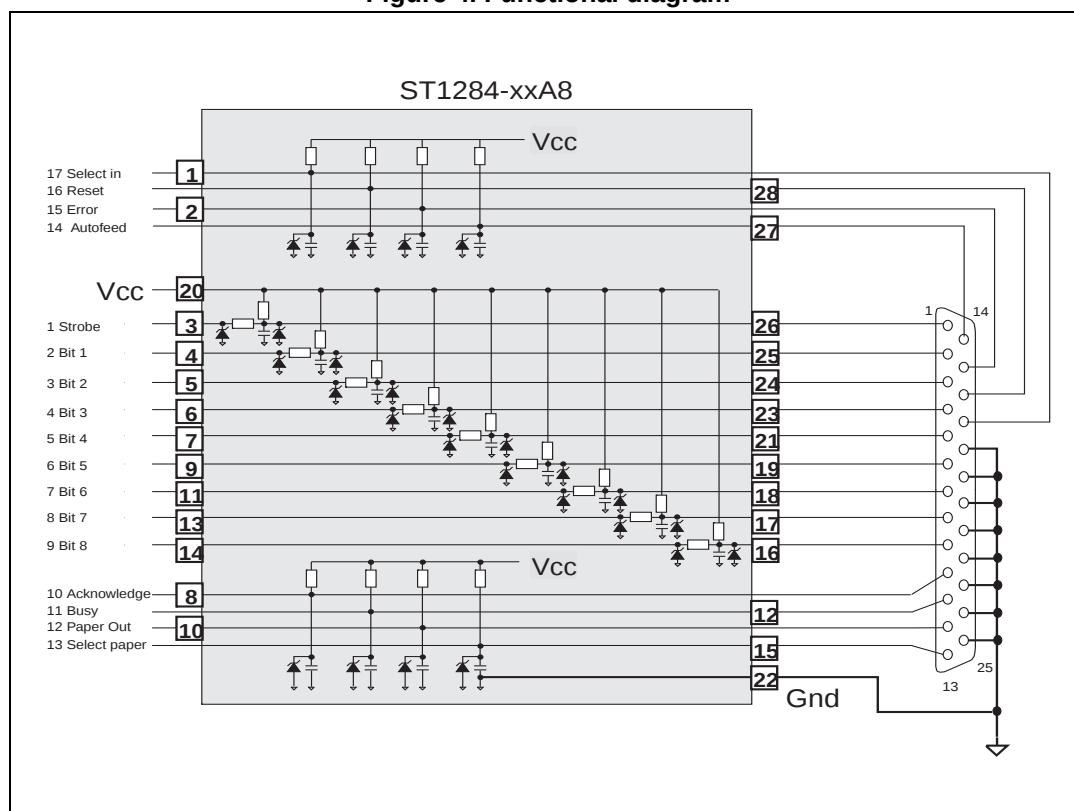
Figure 4. Functional diagram
