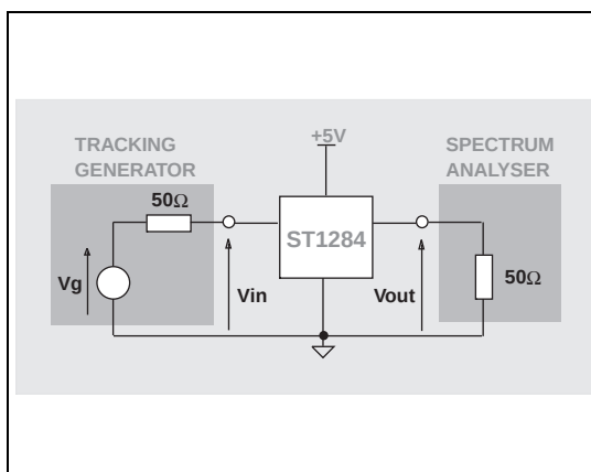
Figure 5. Measurement conditions
