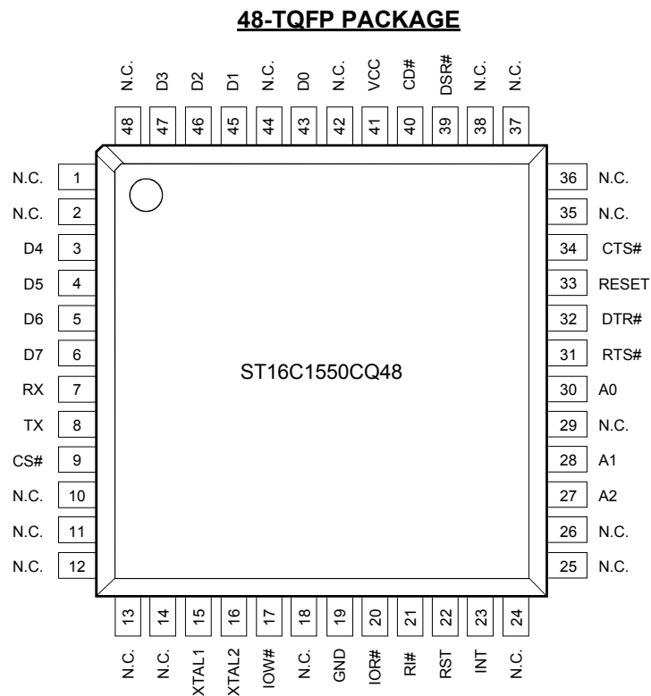
FIGURE 2. ST16C1550 PINOUTS
