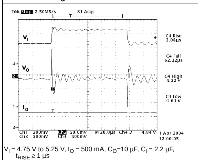
Figure 22. Line transient
