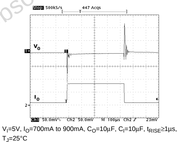
Figure 20. V_O change with step load change I_O = 700 to 900 mA
