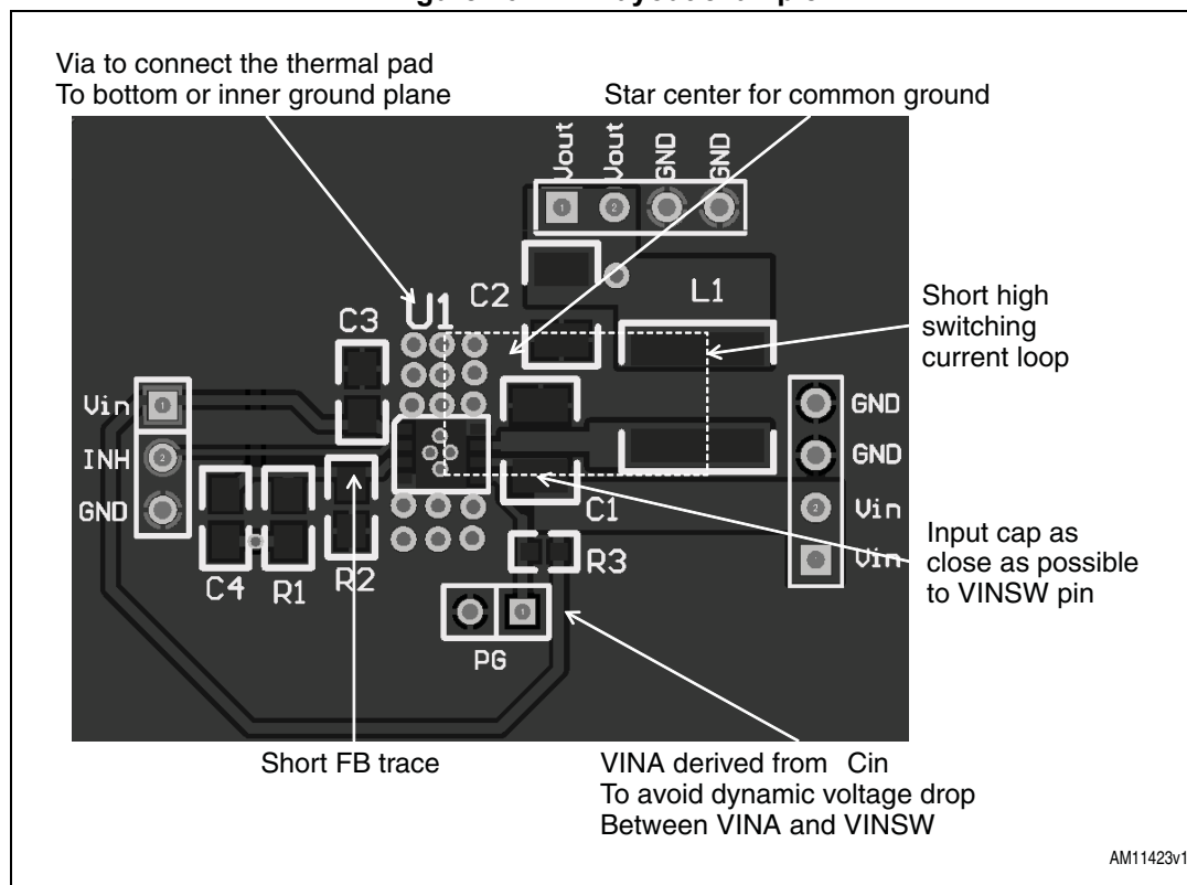
Figure 10. PCB layout example
