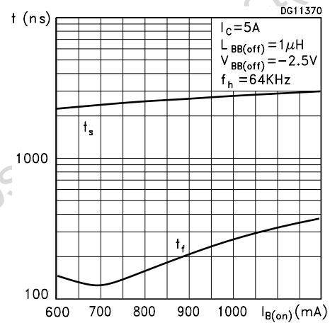
Inductive Load Switchin Times
